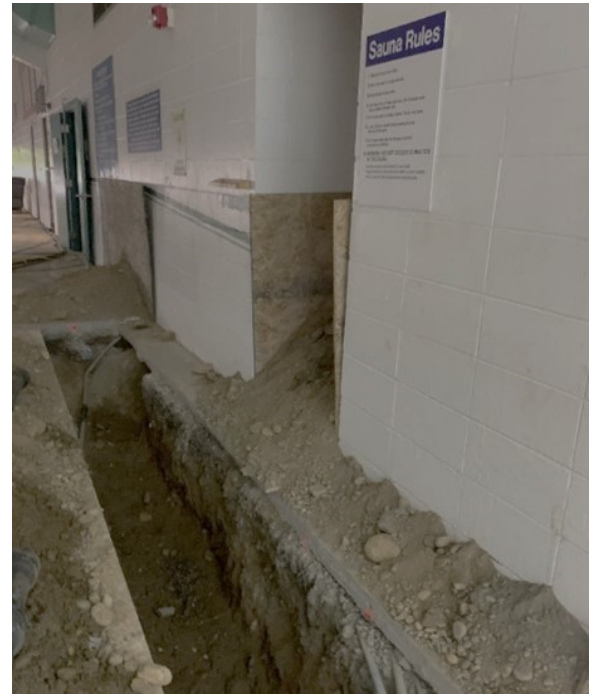
(Above left and right) Demo to pool deck outside of sauna to prepare for the replacement of old and damaged drainage pipes.
