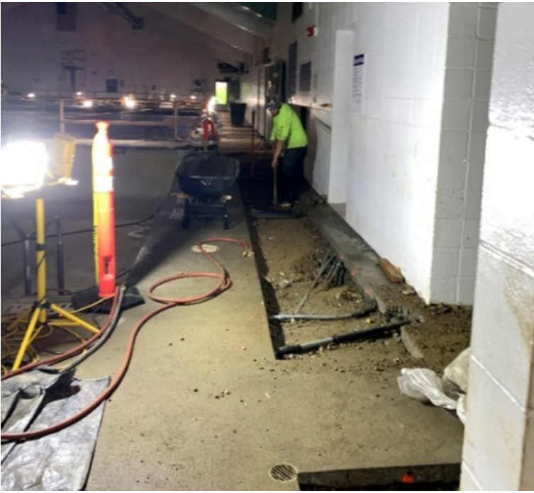
(Above left and right) Demo to pool deck outside of sauna to prepare for the replacement of old and damaged drainage pipes.
