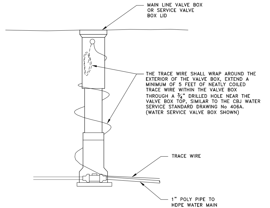
3 MAIN LINE VALVE & SERVICE VALVE TRACE WIRE TERMINATION DETAIL N.T.S.
