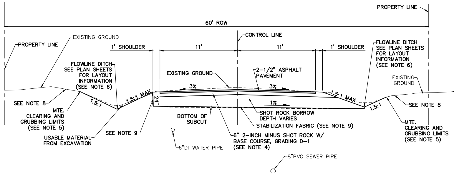
TYPICAL SECTION HERON WAY NTS
