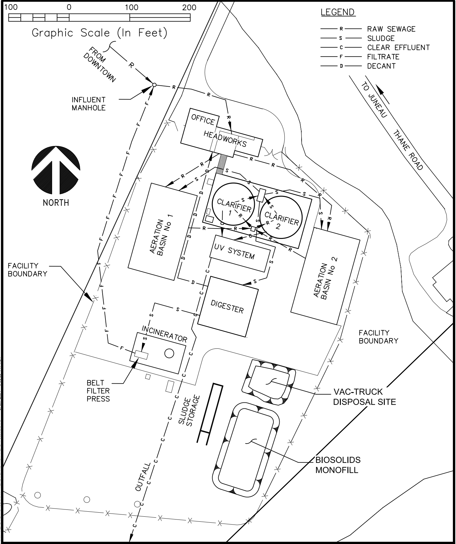
FIGURE 1 JDWWTP SITE PLAN
