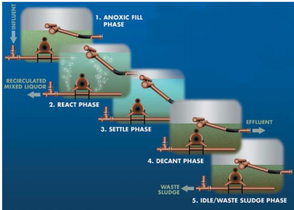
Figure 9. SBR Cycles
