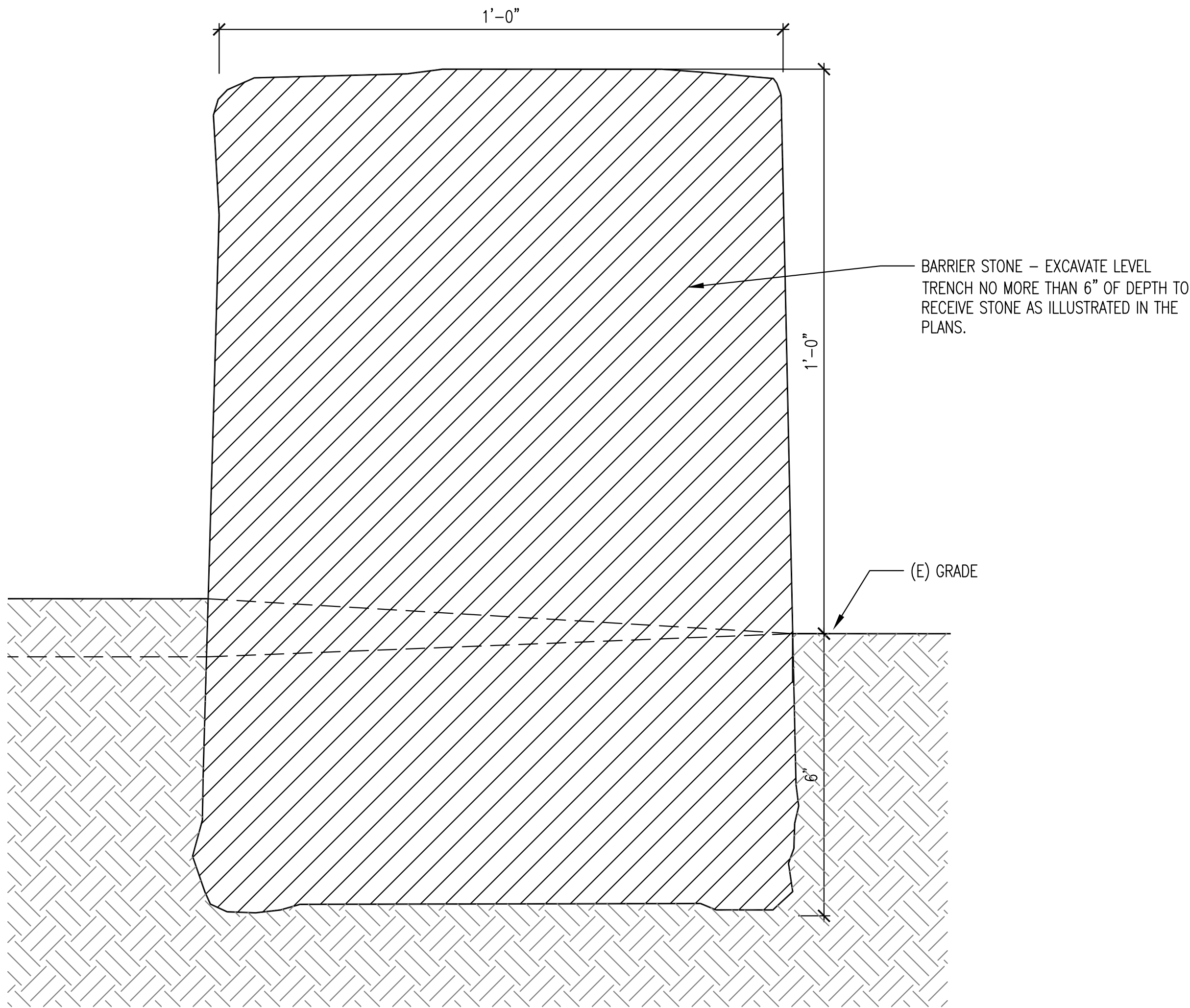
② STONE PLACEMENT ON GRADE
