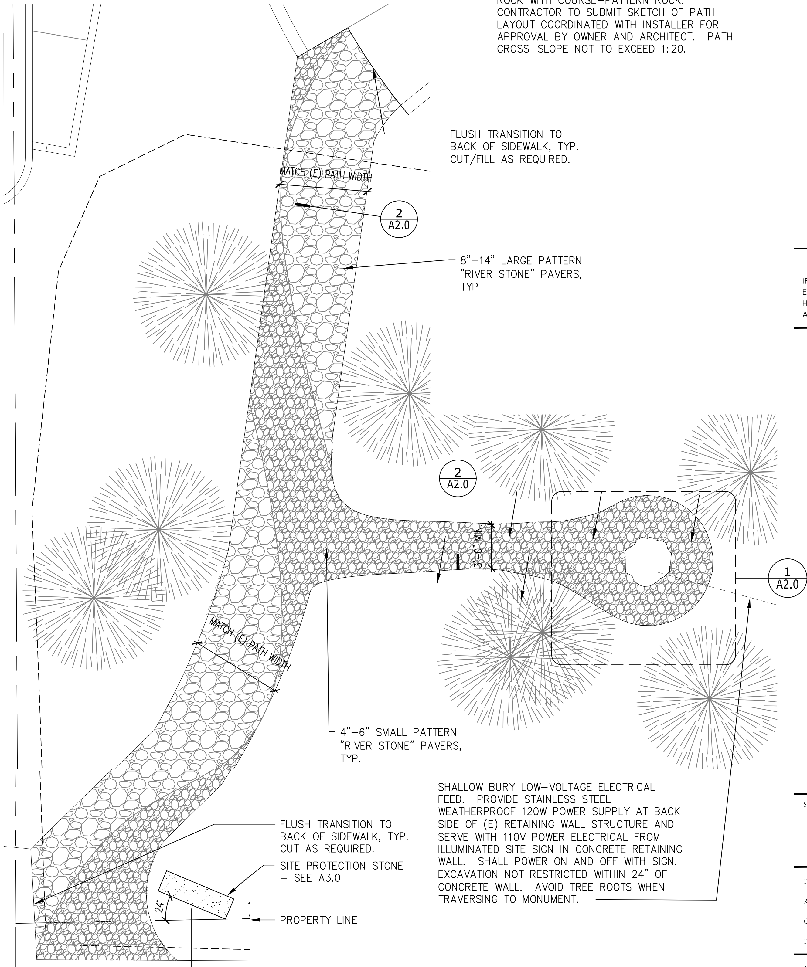
3 RIVER PATH AND MEMORIAL 1/4" = 1'-0"
