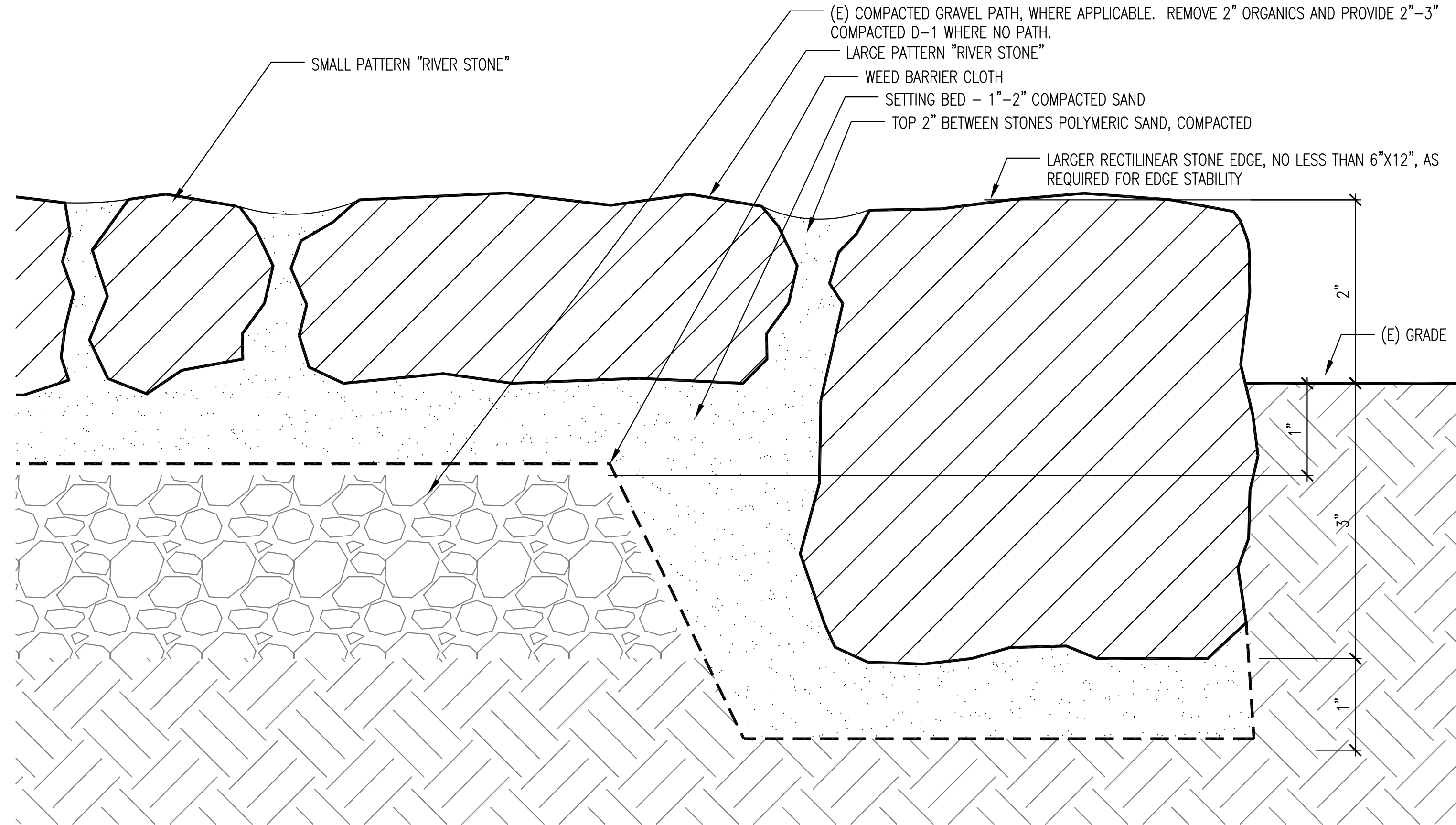
2 RIVER PATH EDGE DETAIL
