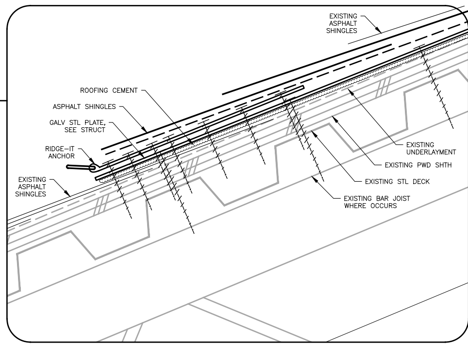
ENLARGED VIEW RIDGE-IT W/1 SINGLE D-RING ANCHOR
