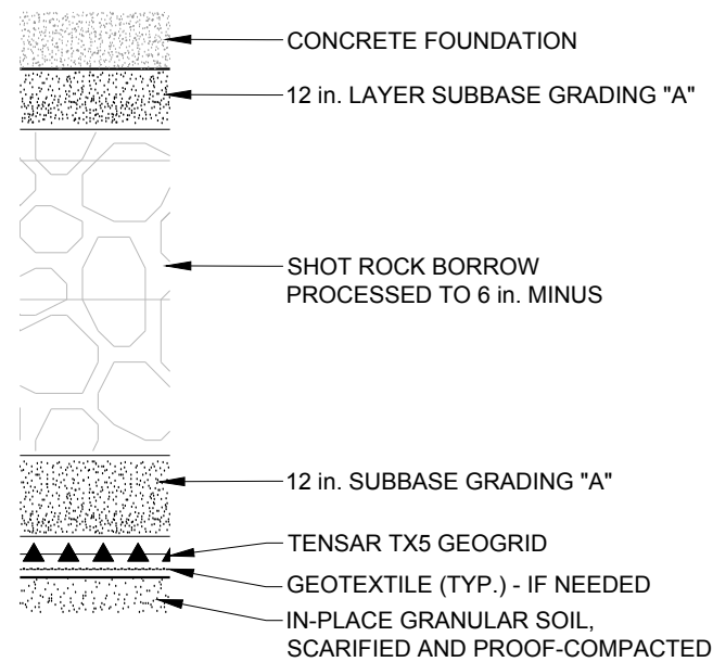
1 SECTION DETAIL
