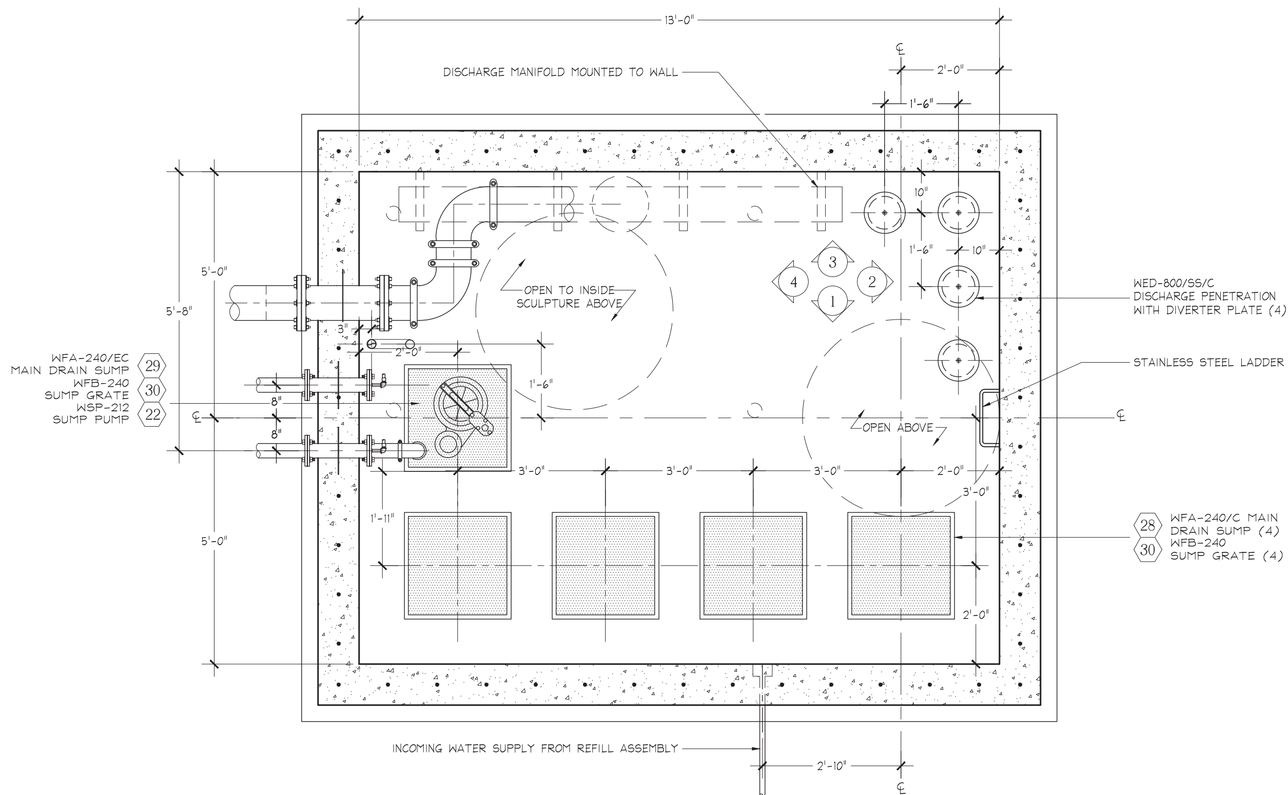
Under Pool Access Chamber Plan Scale 1/2" = 1' - 0"
