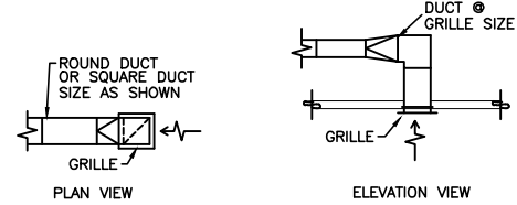
RETURN/EXHAUST GRILLE CONNECTIONS
