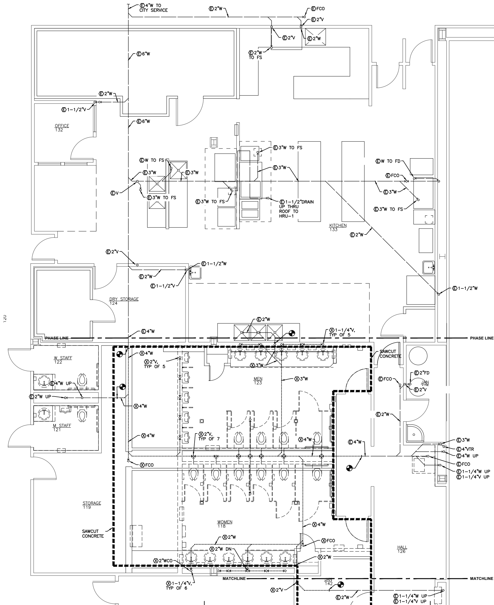
2 FAMILY TR SCALE: 0 2' 4' 8' PROJECT NORTH
