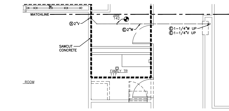
2 FAMILY TR SCALE: 0 2' 4' 8' PROJECT NORTH
