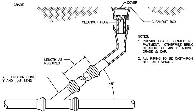
2 YARD CLEAN OUT DETAIL NO SCALE
