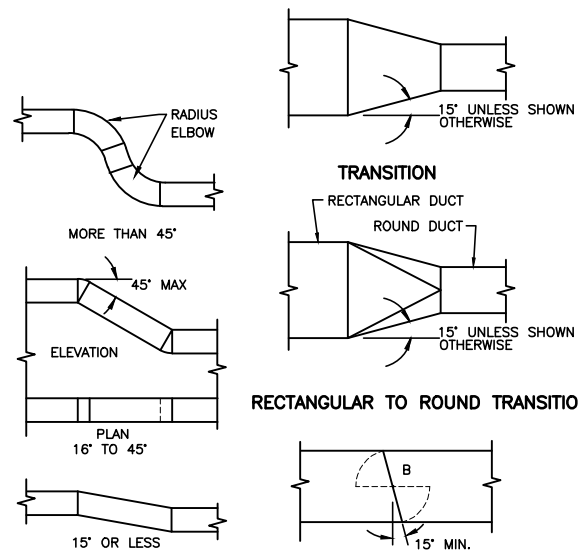
RECTANGULAR AND ROUND DUCTS
