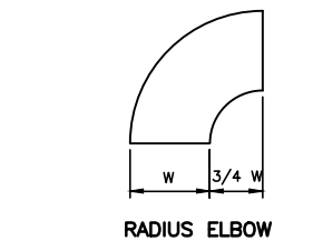
RADIUS ELBOW
