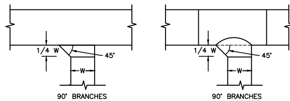
BRANCH DUCT CONNECTIONS
