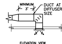
DIFFUSER CONNECTIONS
