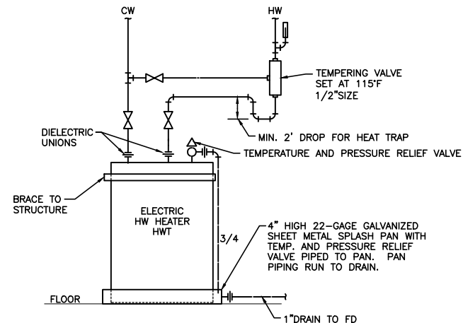
3 ELECTIC HOT WATER HEATER DETAIL NO SCALE
