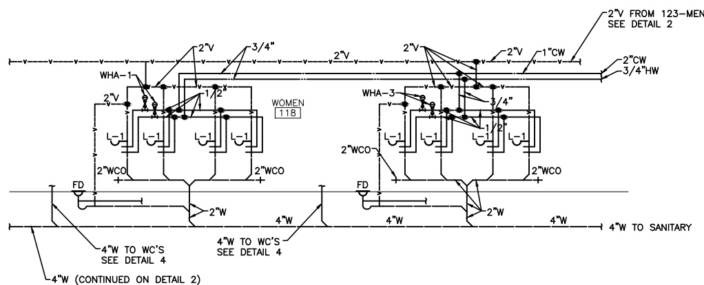
3 PLUMBING DIAGRAM - NORTH TOILETS - PARTIAL
