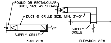
SUPPLY GRILLE CONNECTIONS
