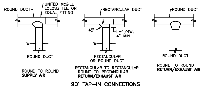
90° TAP-IN CONNECTIONS
