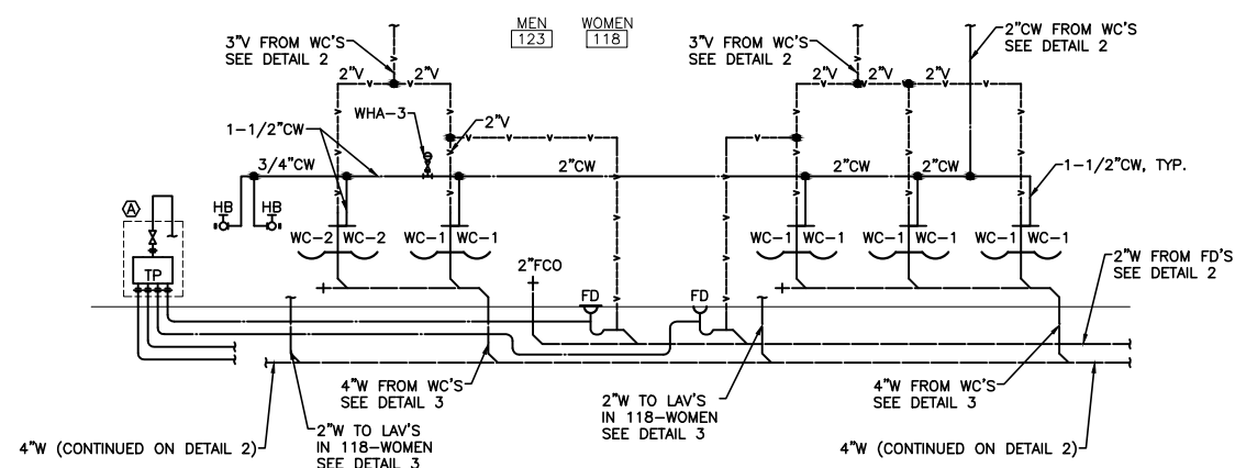
4 PLUMBING DIAGRAM - NORTH TOILETS - PARTIAL
