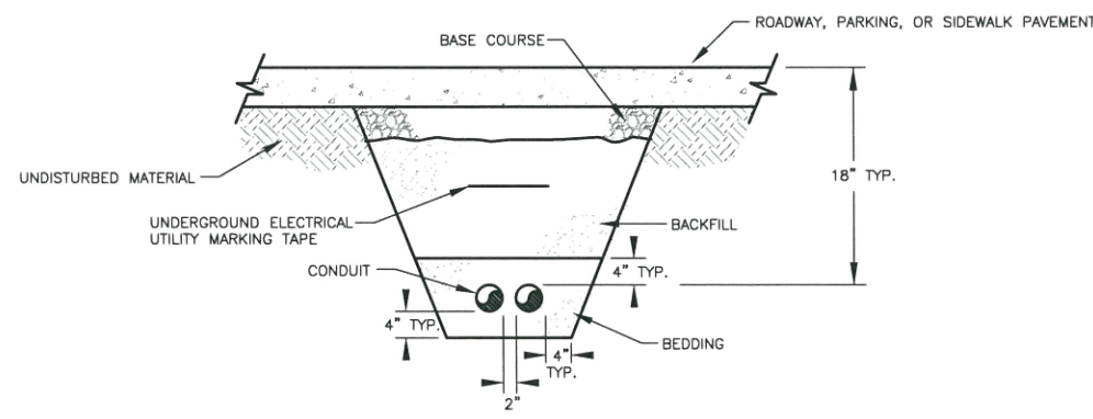
3 TRENCH - SECONDARY NO SCALE
