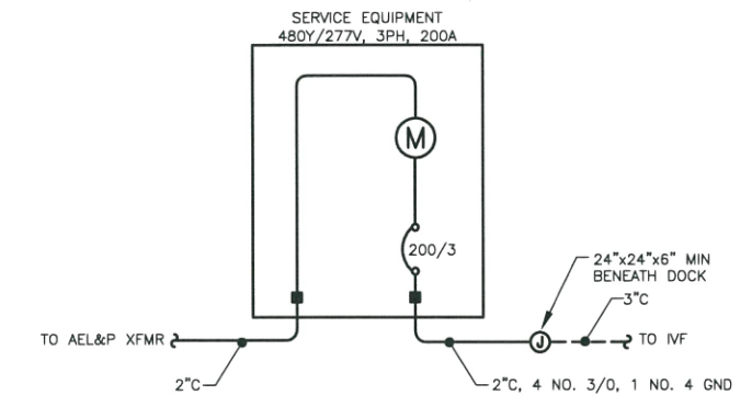
5 SINGLE LINE DIAGRAM - IVF SERVICE NO SCALE
