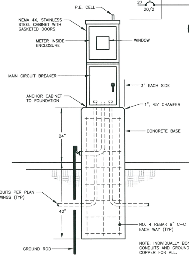
4 DETAIL - IVF SERVICE EQUIPMENT NO SCALE
