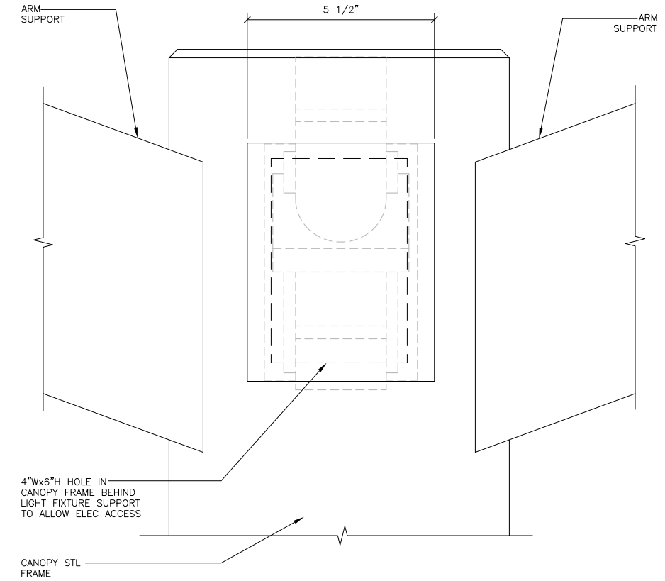
1 LIGHT FIXTURE SUPPORT (SIDE) 10089/X_A4.03-1
