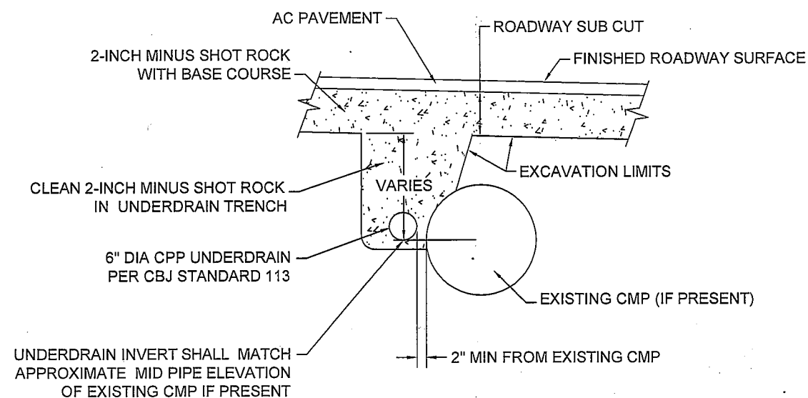
UNDERDRAIN SECTION NTS
