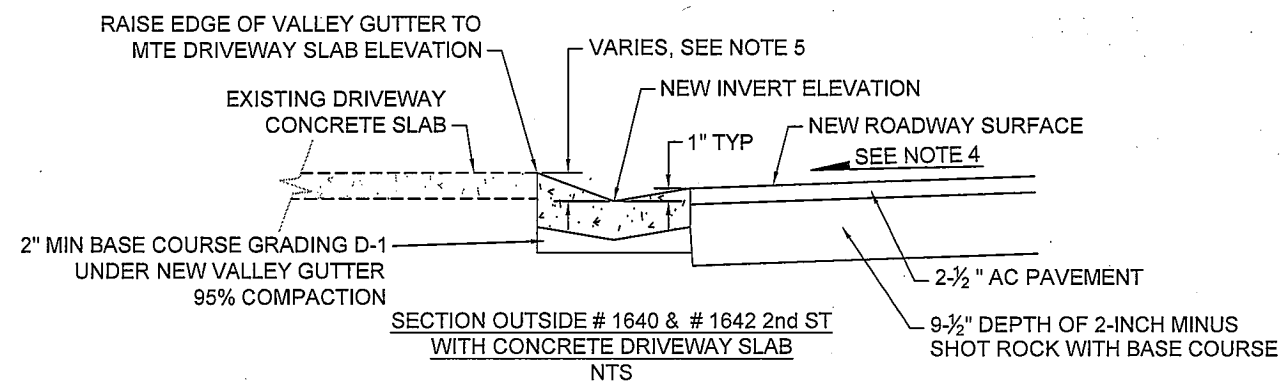
NEW VALLEY GUTTER SECTIONS NTS
