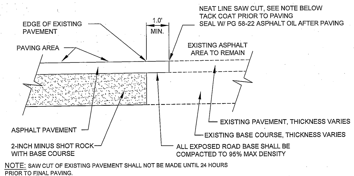
PAVEMENT MATCH JOINT DETAIL NTS
