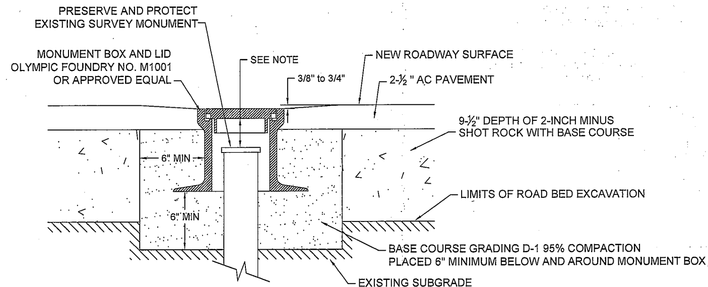
MONUMENT BOX SECTION NTS
