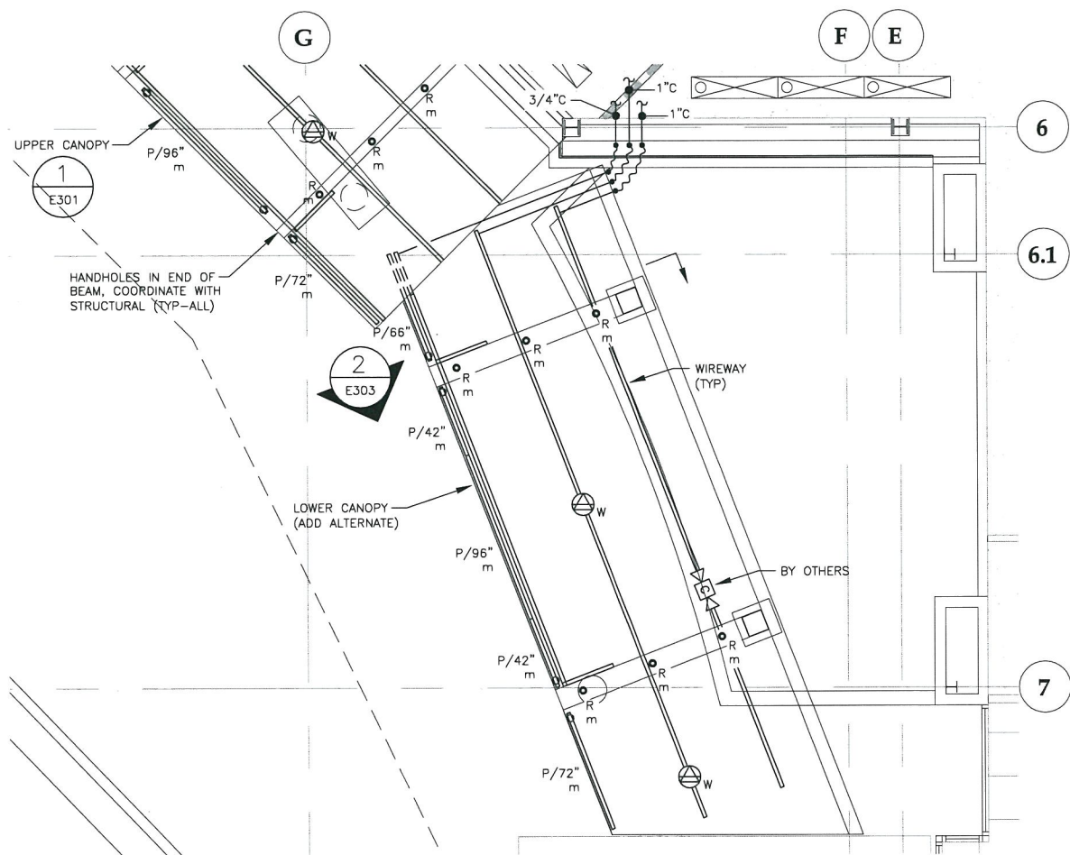
1 ENLARGED 1st FLOOR PLAN - LIGHTING & LOW VOLTAGE
