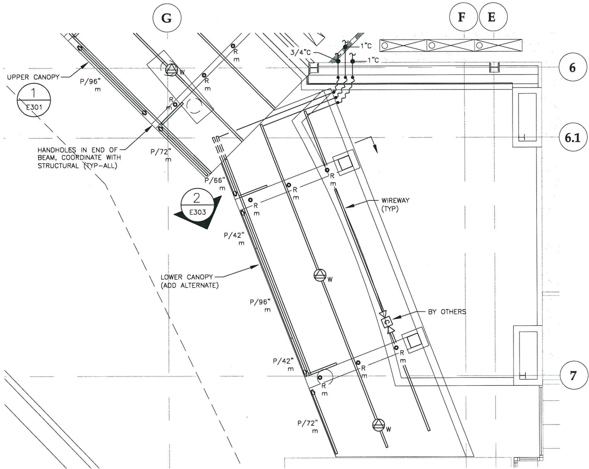
1 ENLARGED 1st FLOOR PLAN - LIGHTING & LOW VOLTAGE
