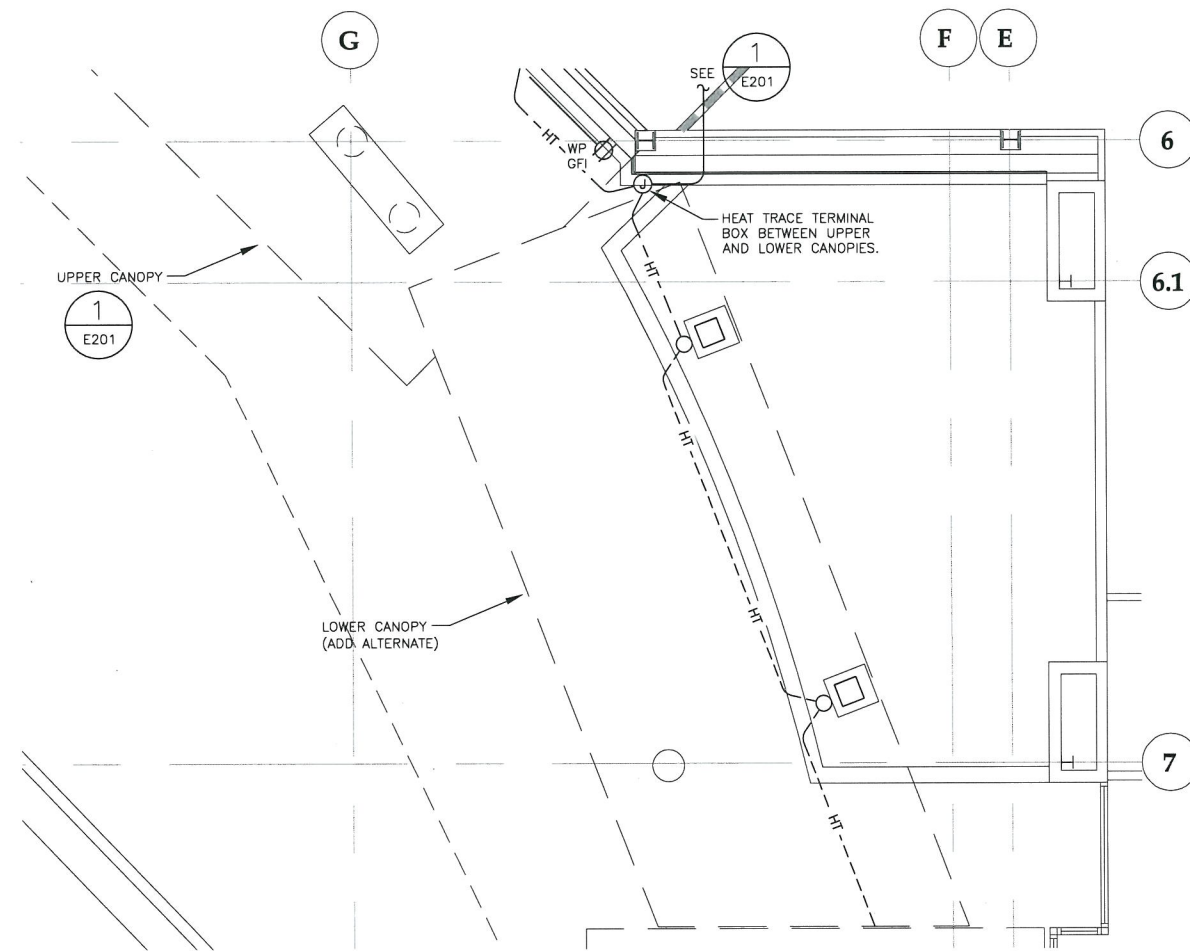
1 ENLARGED 1st FLOOR PLAN - POWER
