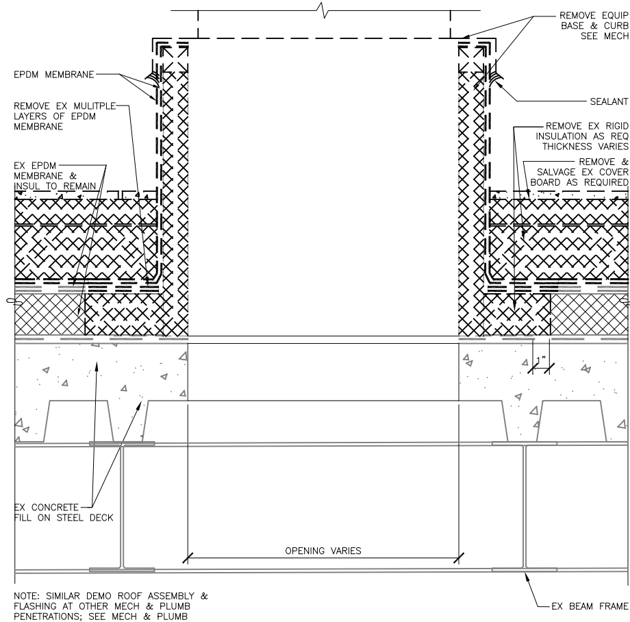
6 DEMO TYPICAL ROOF CURB ASSEMBLY 0859/X_A1801-6 SCALE: 0 3" 6" 1'
