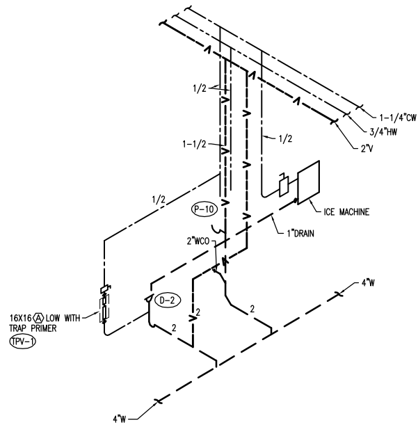
2 PLUMBING DIAGRAM - ICE MACHINE P7.01 P7.01 NONE
