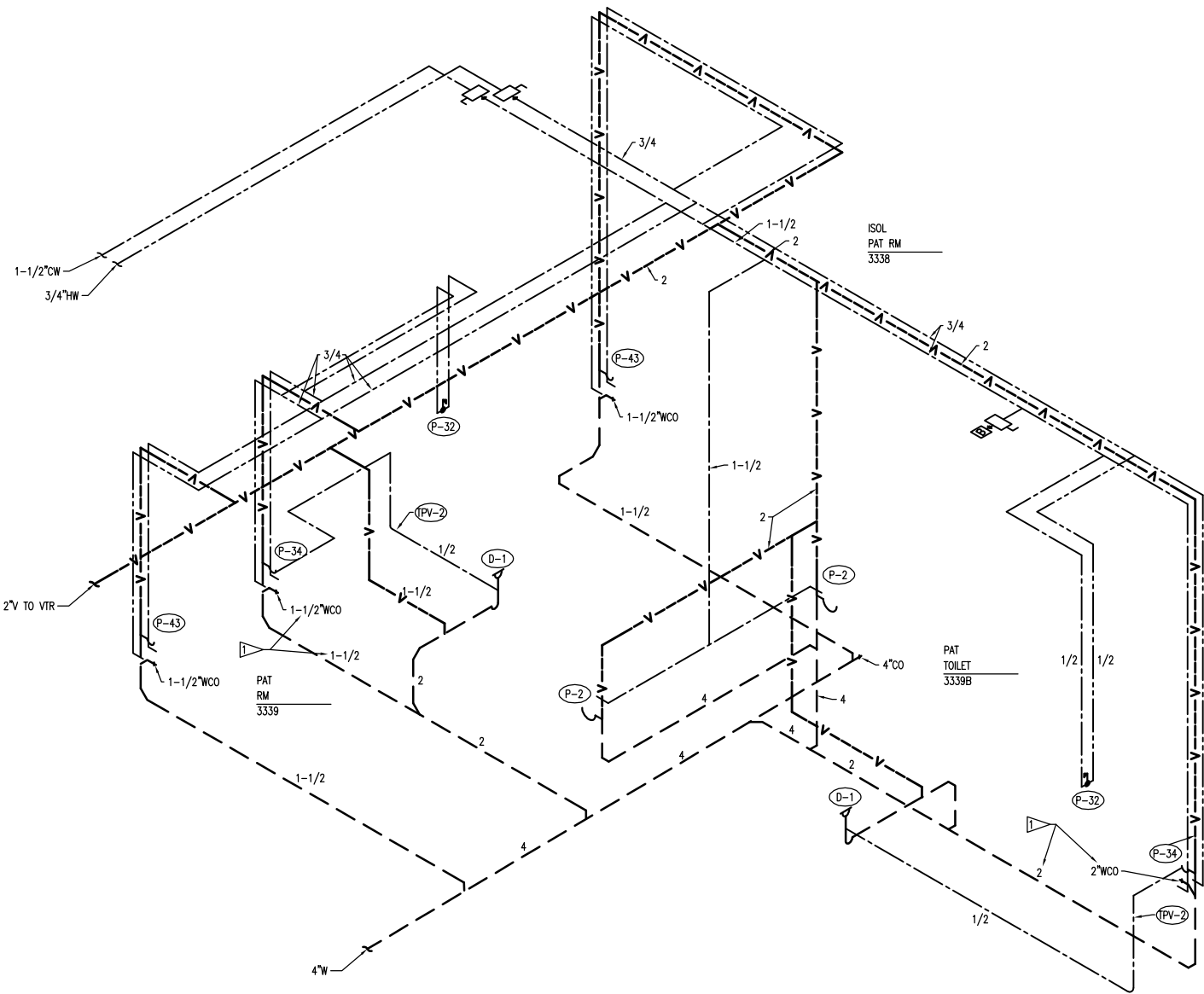
1 PATIENT TOILET ROOMS PLUMBING DIAGRAM - TYPICAL P7.01 P7.01 NONE
