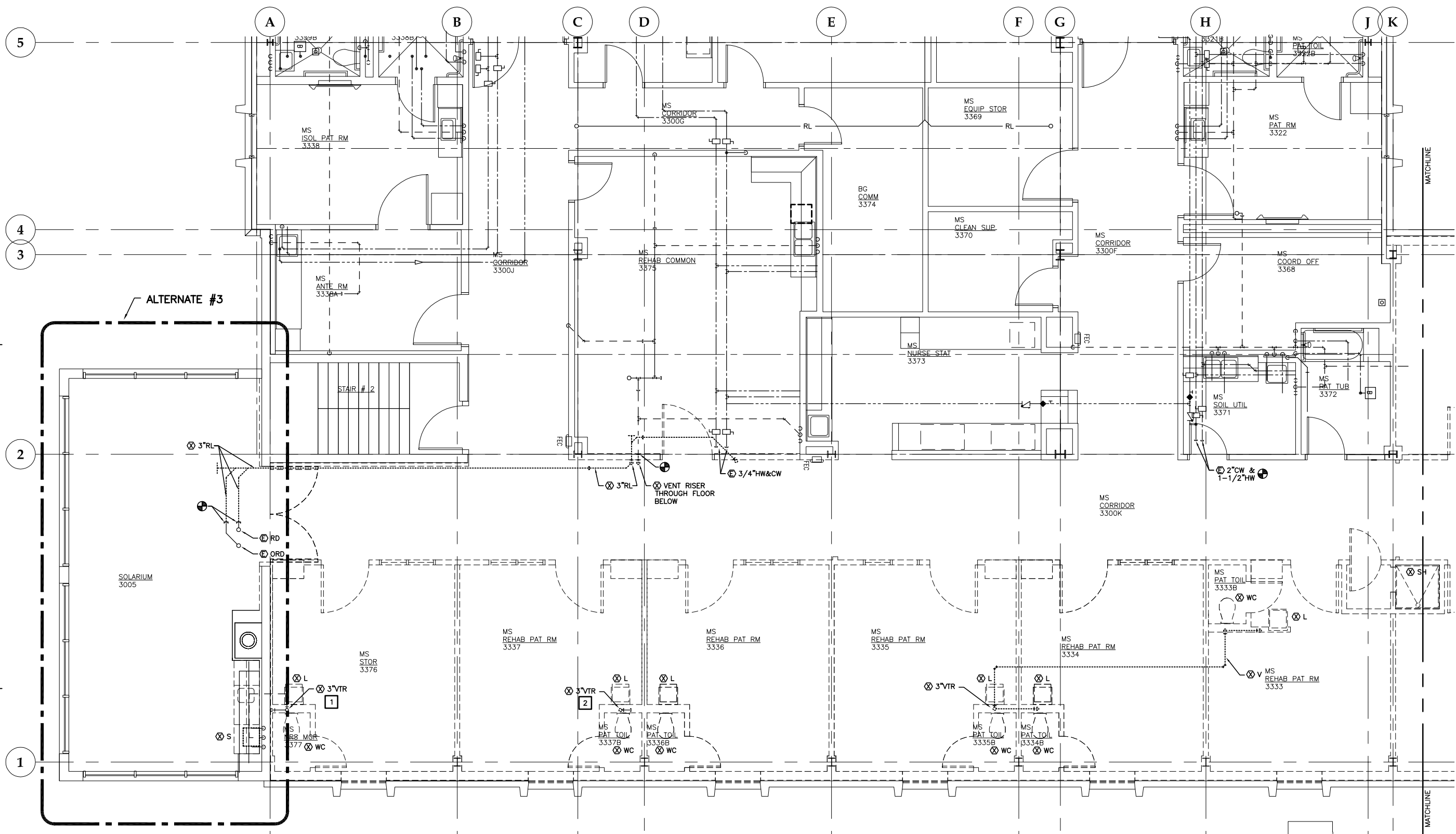
1 DEMOLITION FLOOR PLAN: LEVEL 3 SOUTH - PLUMBING
