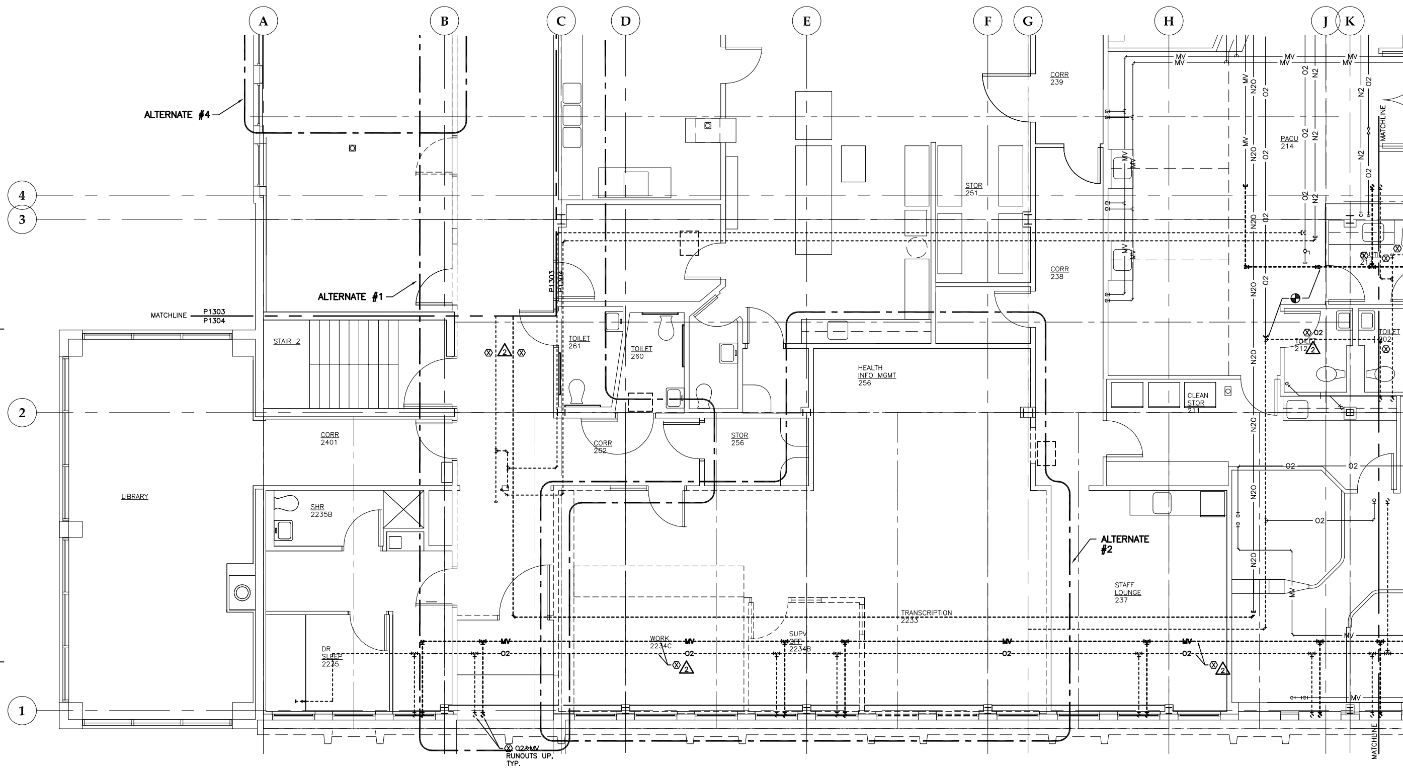
1 DEMOLITION FLOOR PLAN: LEVEL 2 SOUTH - MEDICAL GAS PIPING
