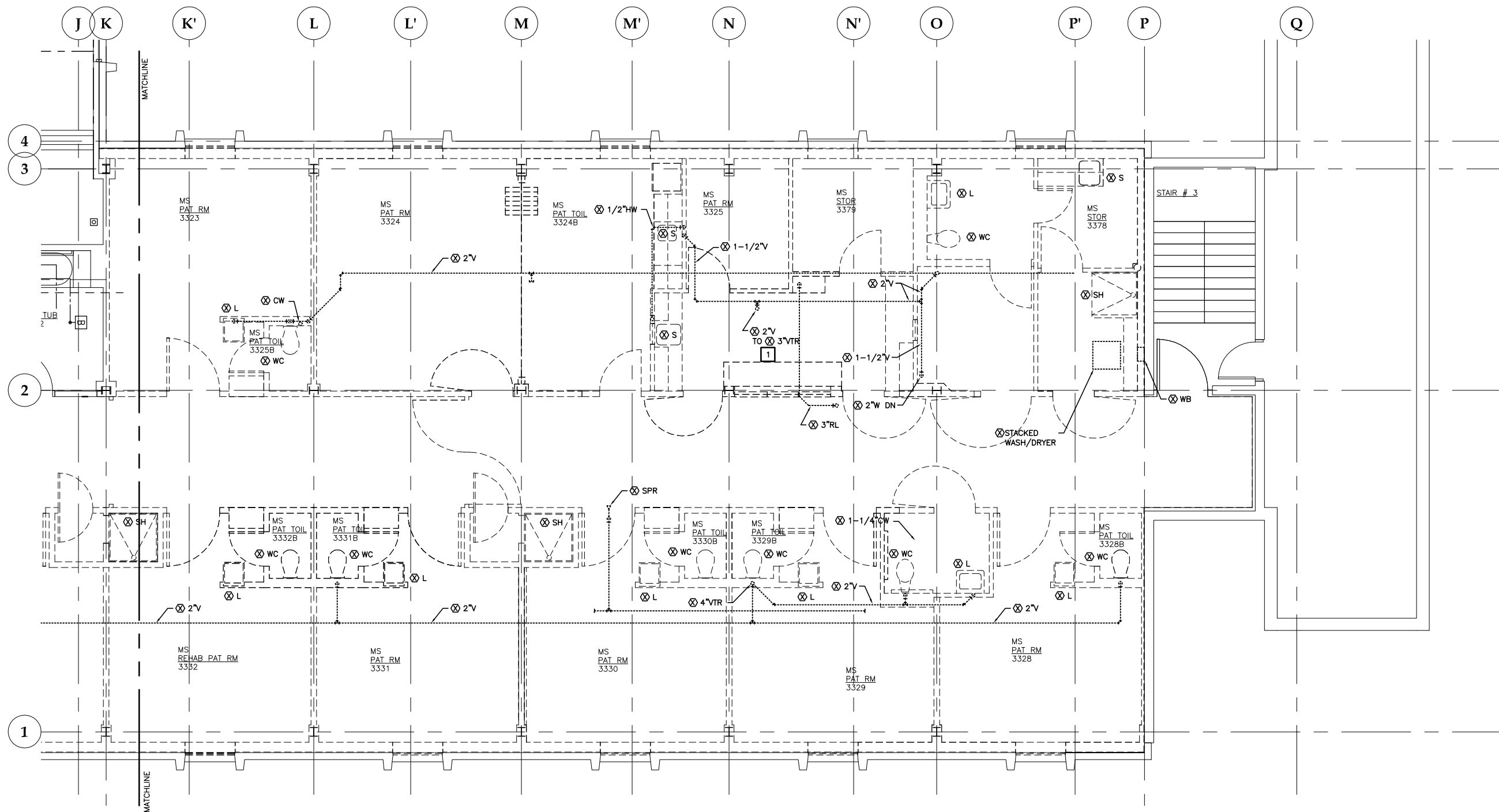
1 DEMOLITION FLOOR PLAN: LEVEL 3 - NORTH PLUMBING SCALE: 0 2' 4' 8'
