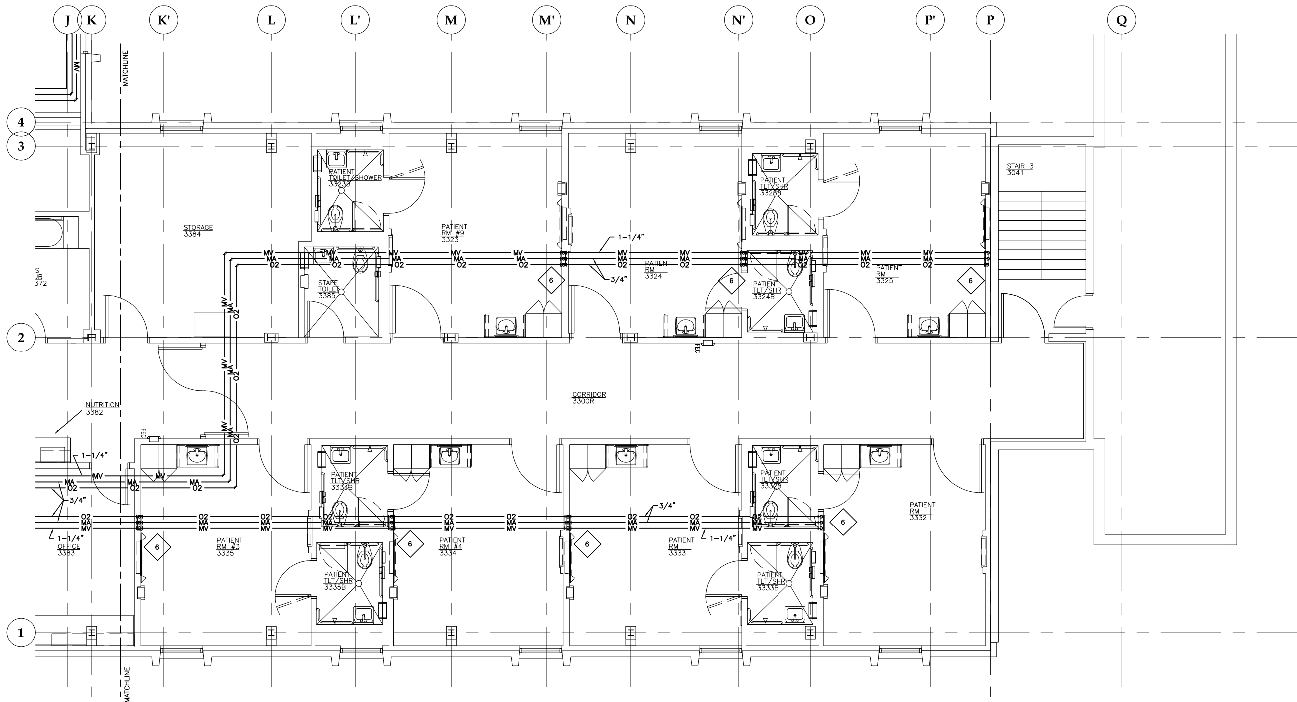
1 FLOOR PLAN: LEVEL 3 - NORTH MEDICAL GAS PIPING SCALE: 0 2' 4' 8'
