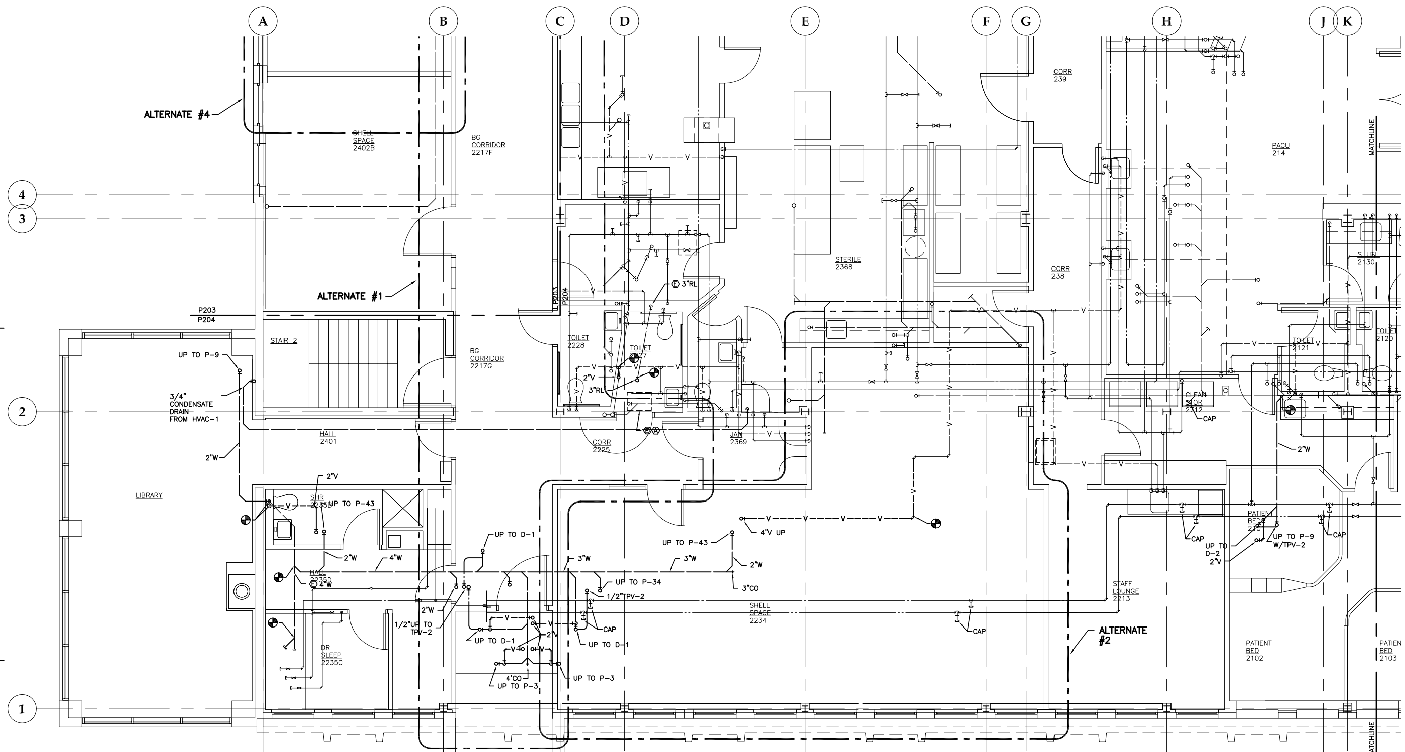
1 FLOOR PLAN: LEVEL 2 SOUTH - PLUMBING
