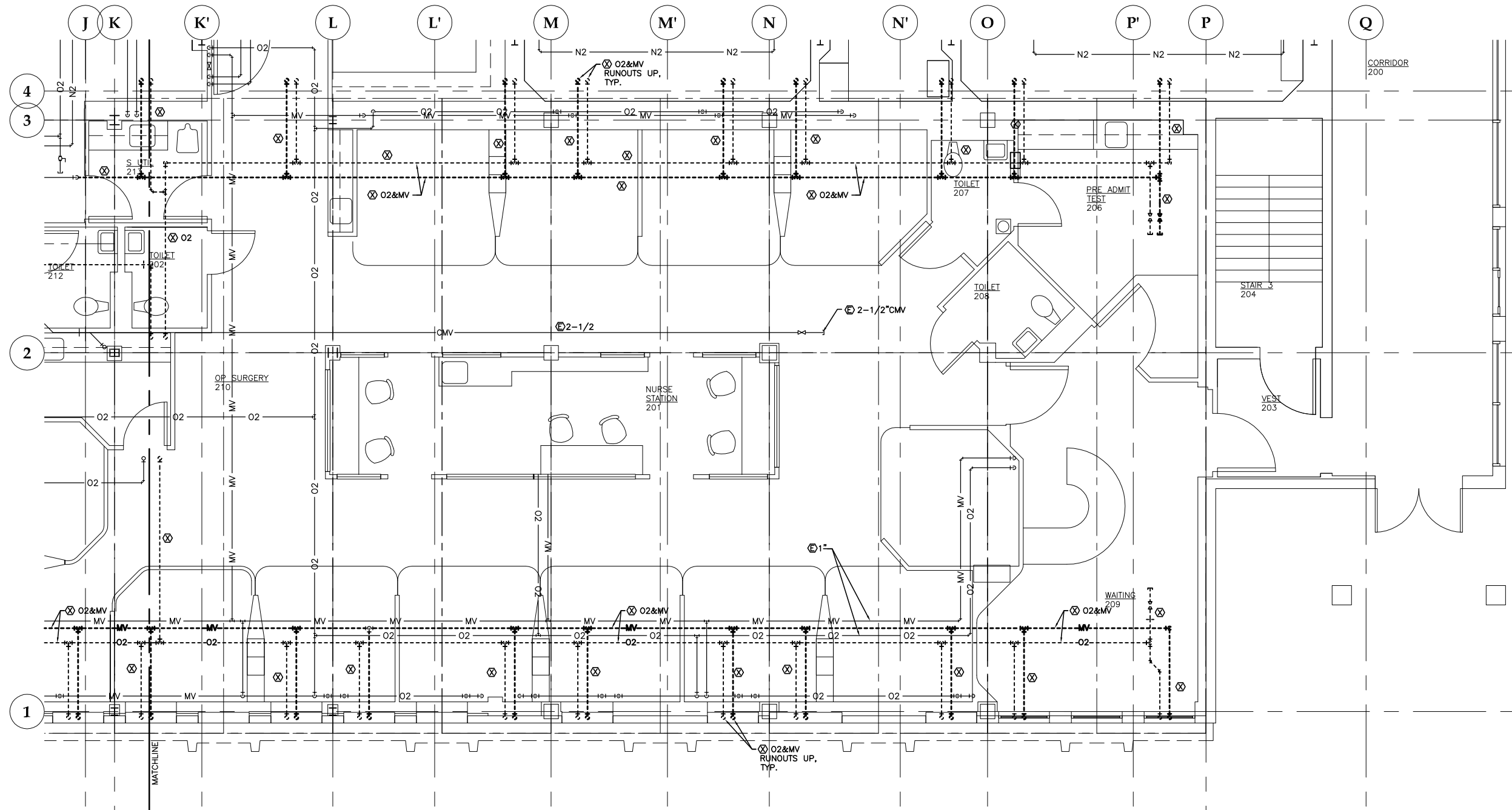
1 DEMOLITION FLOOR PLAN: LEVEL 2 NORTH - MEDICAL GAS PIPING
