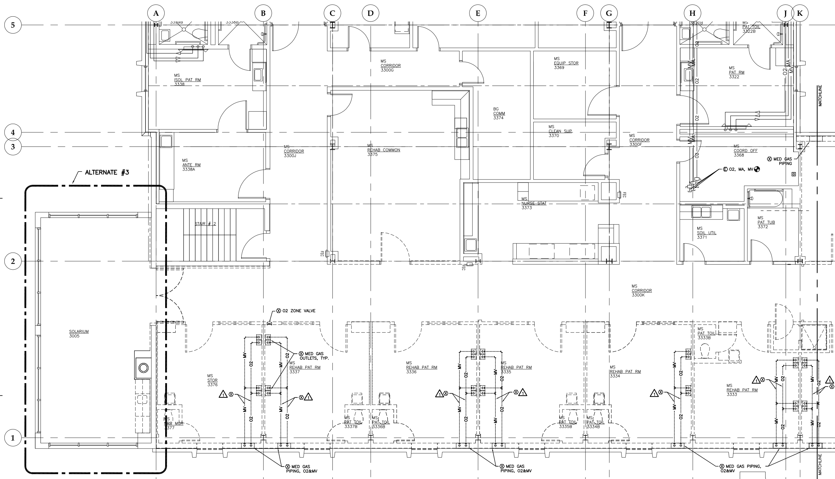
1 DEMOLITION FLOOR PLAN: LEVEL 3 SOUTH - MEDICAL GAS PIPING
