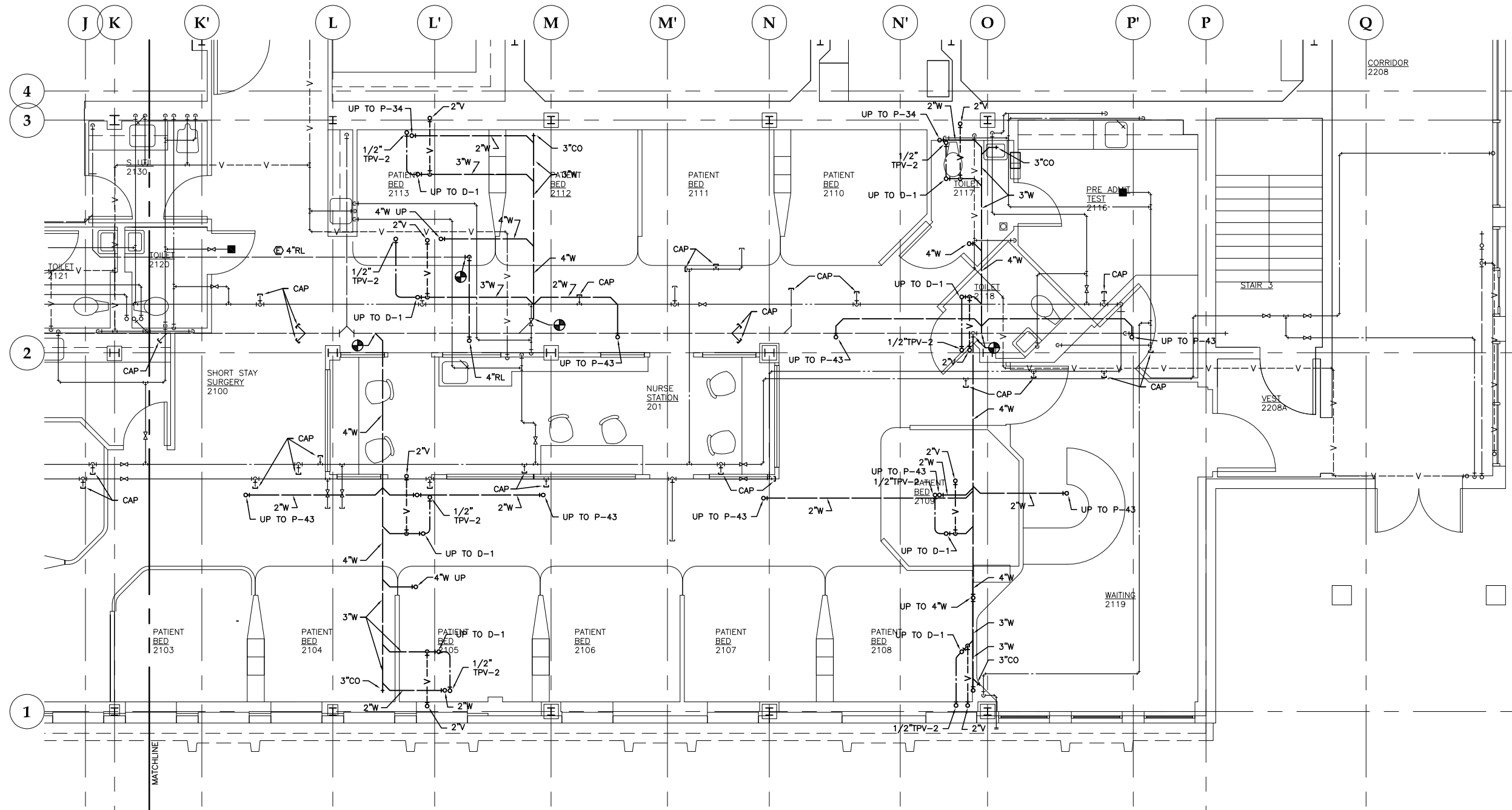
1 FLOOR PLAN: LEVEL 2 NORTH- PLUMBING
