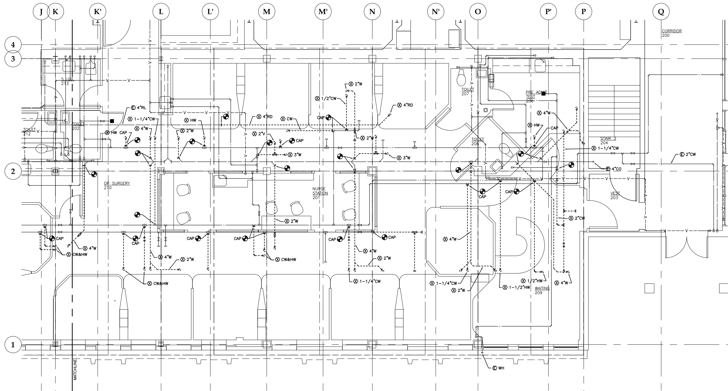
1 DEMOLITION FLOOR PLAN: LEVEL 2 NORTH - PLUMBING
