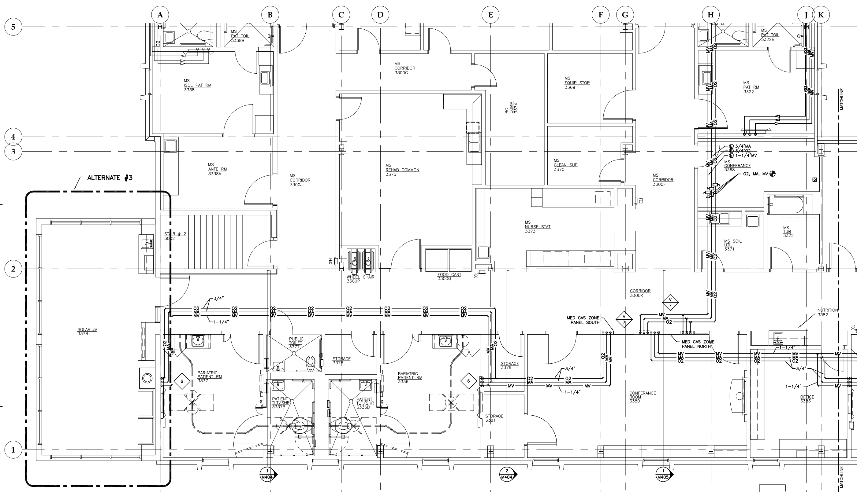
1 FLOOR PLAN: LEVEL 3 SOUTH - MEDICAL GAS PIPING
