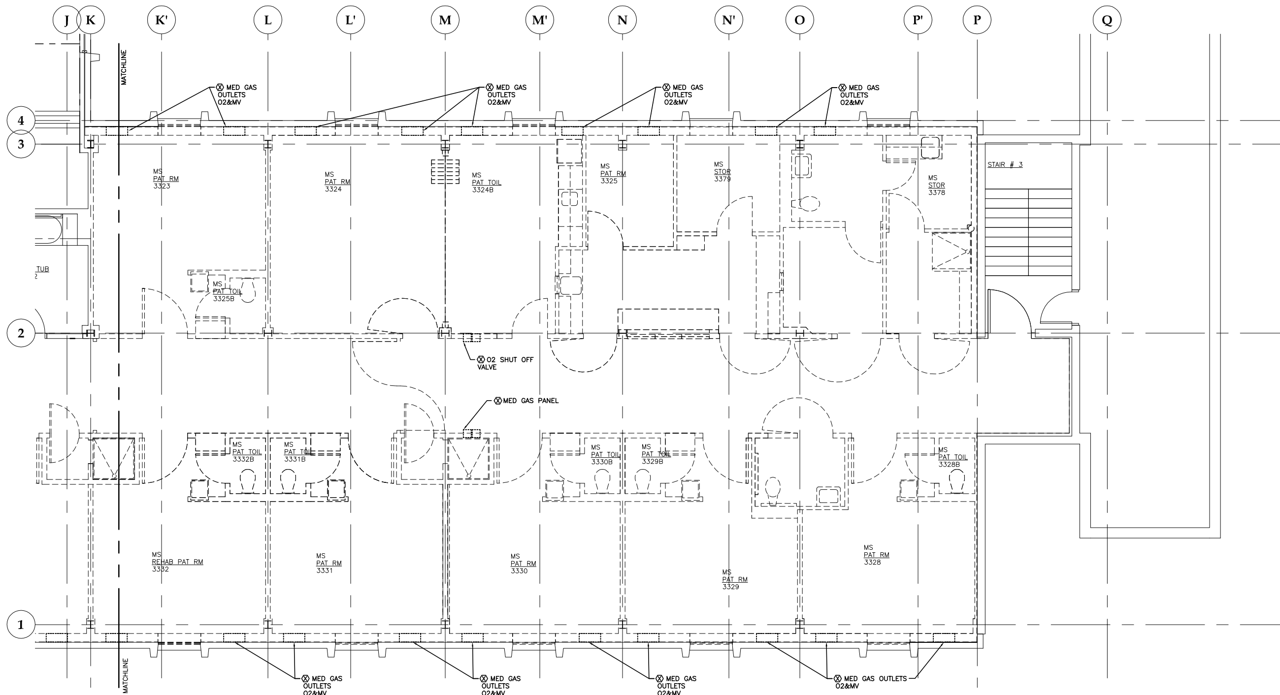
1 DEMOLITION FLOOR PLAN: LEVEL 3 NORTH - MEDICAL GAS PIPING SCALE: 0 2' 4' 8'
