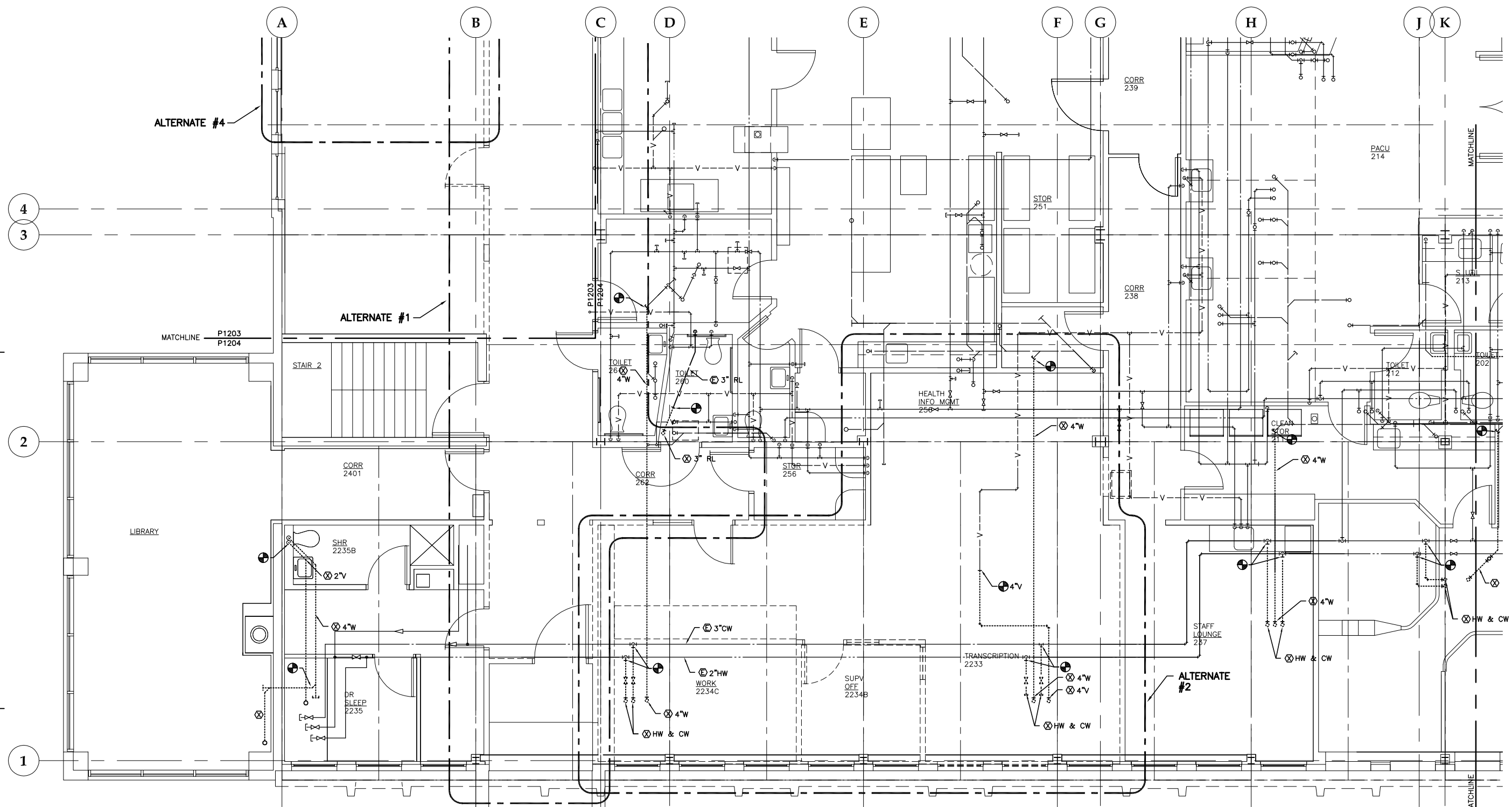
1 DEMOLITION FLOOR PLAN: LEVEL 2 SOUTH - PLUMBING
