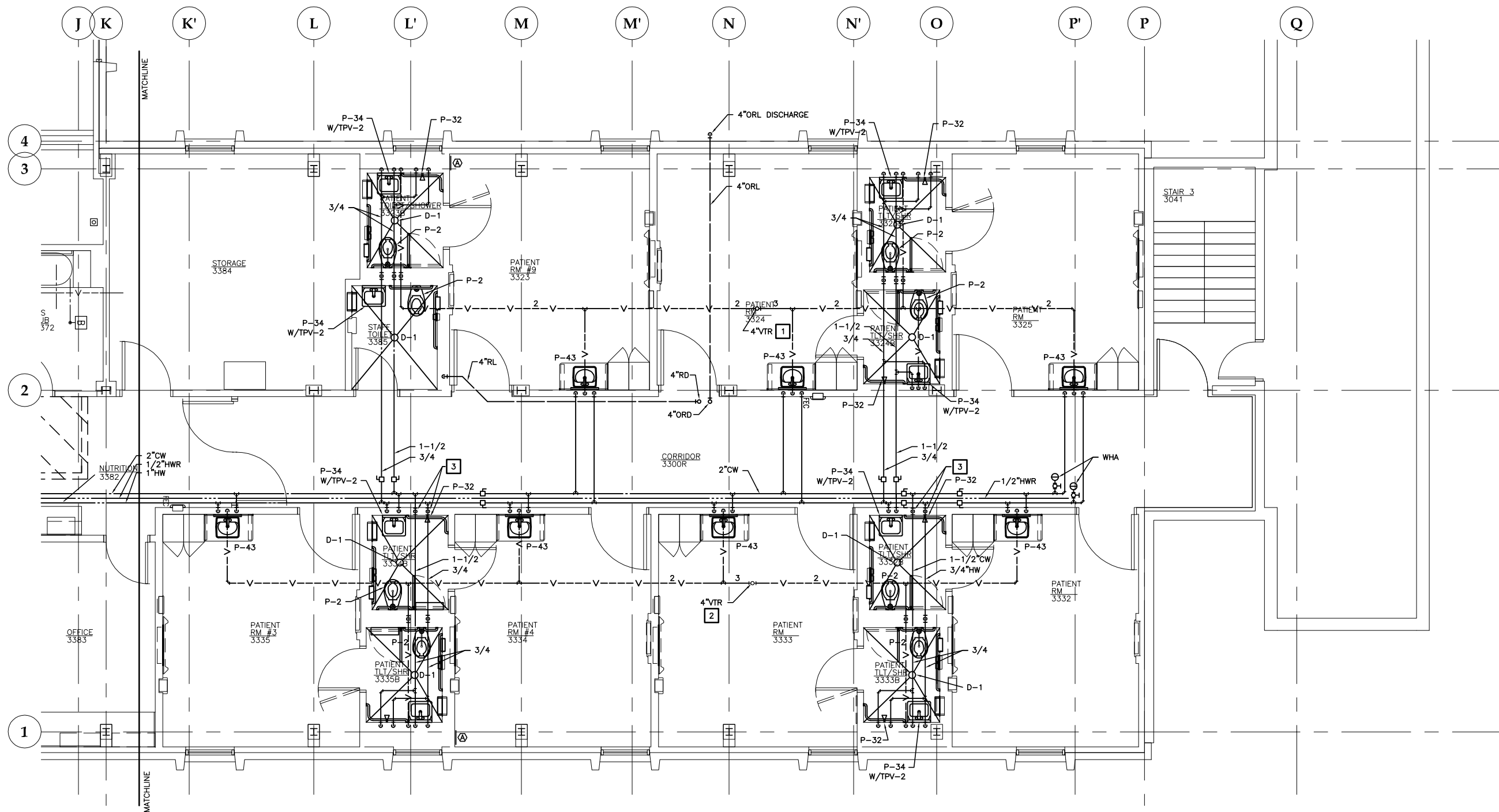
1 FLOOR PLAN: LEVEL 3 - NORTH PLUMBING
