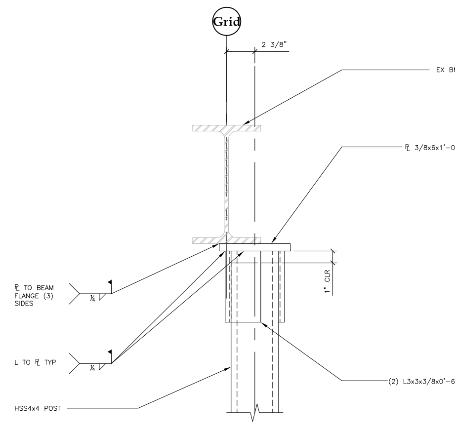
6 HSS POST TO BEAM 0859-A804-6 SCALE: 0 3" 6" 1'
