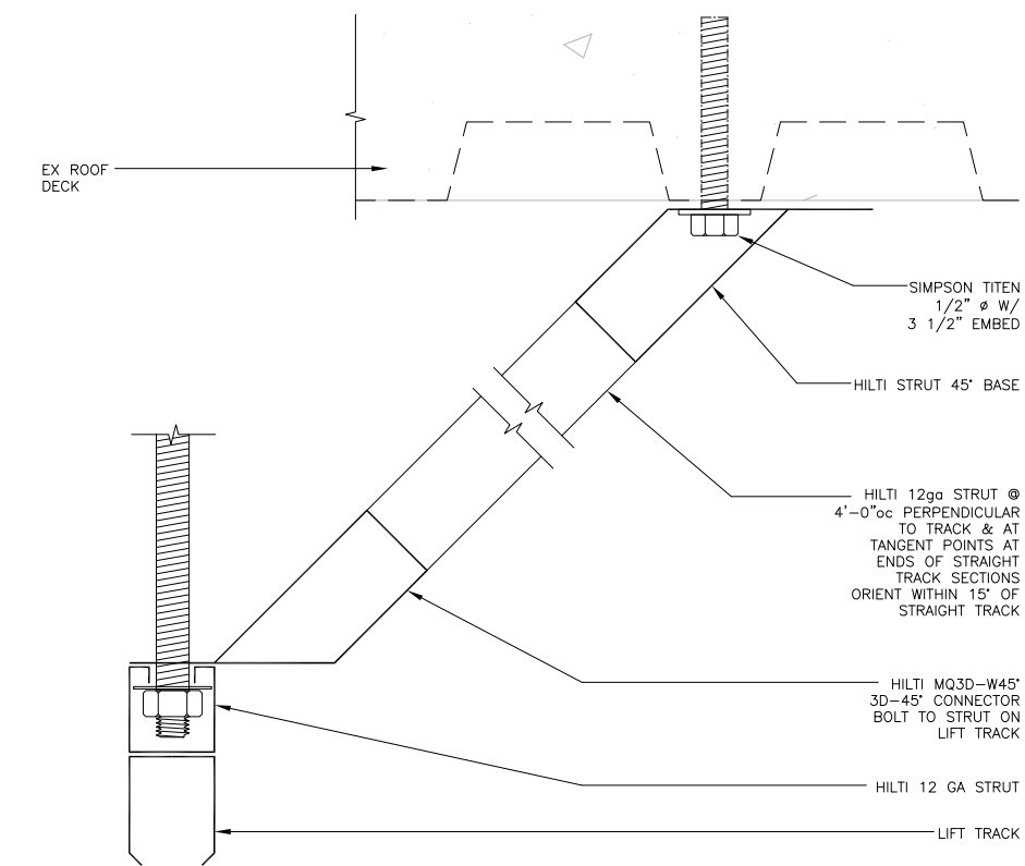
5 LIFT TRACK BRACING 0859/X_A803-5 SCALE: 0 3" 6"
