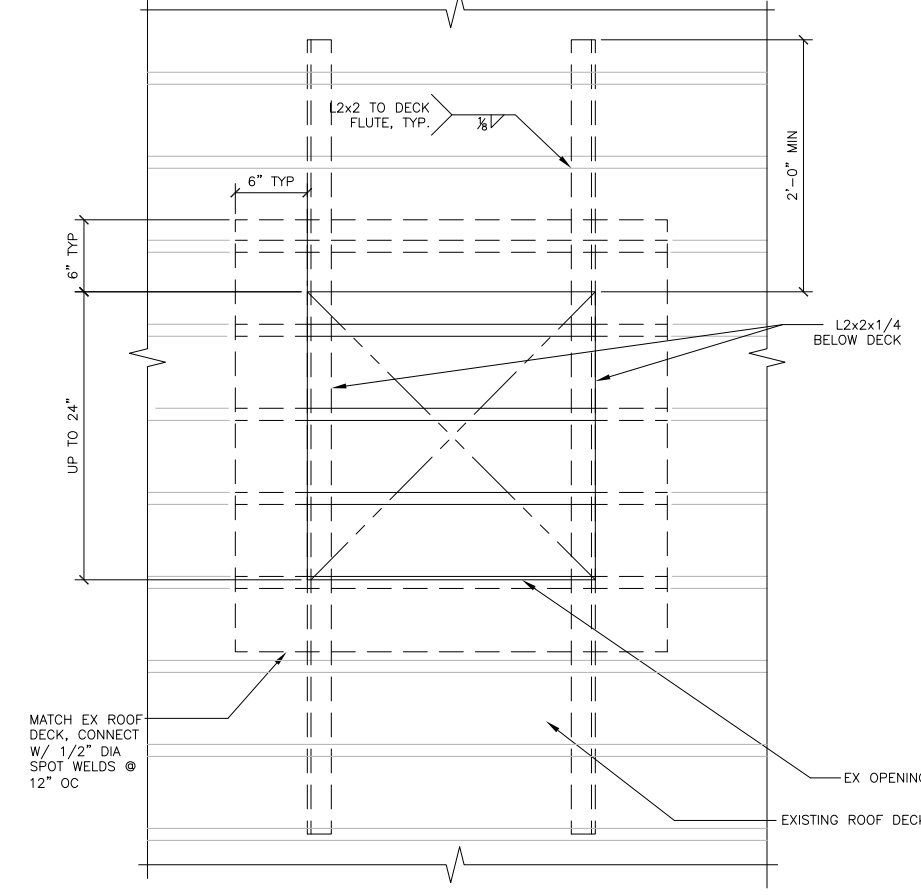
3 EXISTING ROOF OPENING INFILL 0859/A804-3 SCALE: 0 6" 1' 2'
