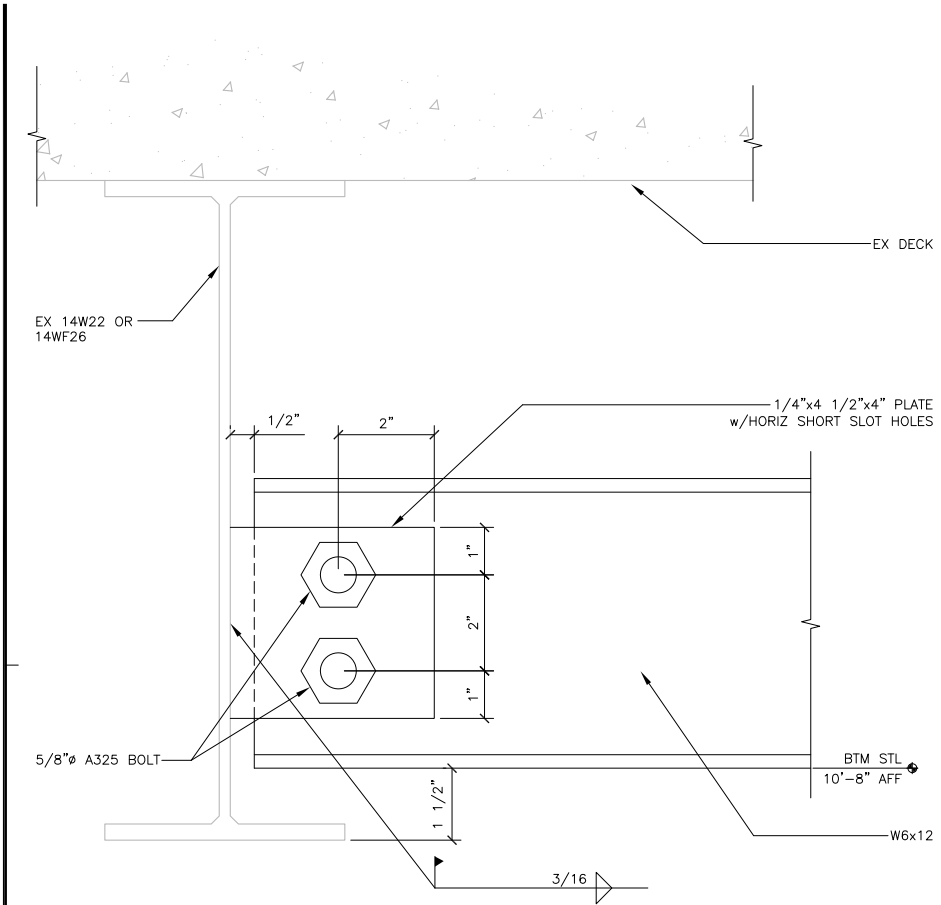
1 W6 TO 14WF DETAIL 0859/X_A803-1 SCALE: 0 3" 6"
