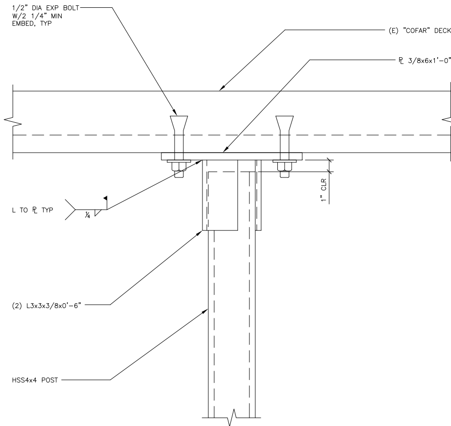
5 TOP HSS POST TO SLAB 0859/A804-5 SCALE: 0 3" 6" 1'
