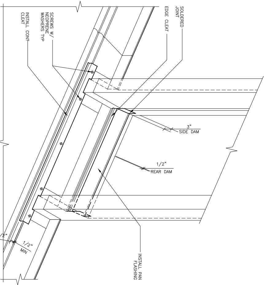
6 WINDOW REPLACEMENT SILL DETAIL
