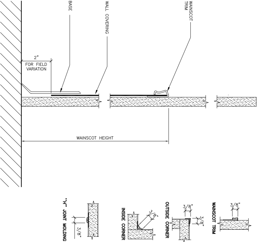
5 WALL COVERING - TYPICAL
