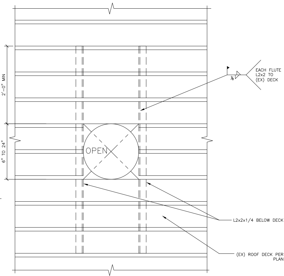
1 TYPICAL ROOF OPENING 0859/A804-1 SCALE: 0 6" 1' 2'
