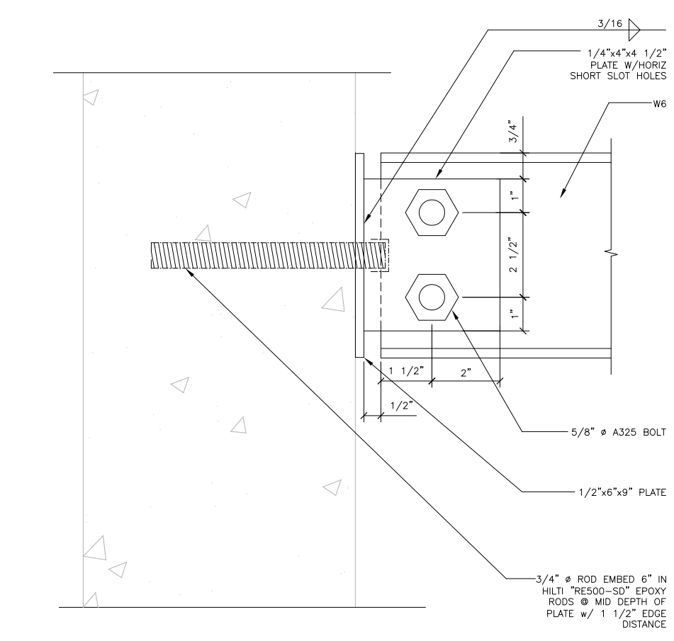
3 W6 TO WALL DETAIL 0859/X_A803-3 SCALE: 0 3" 6"
