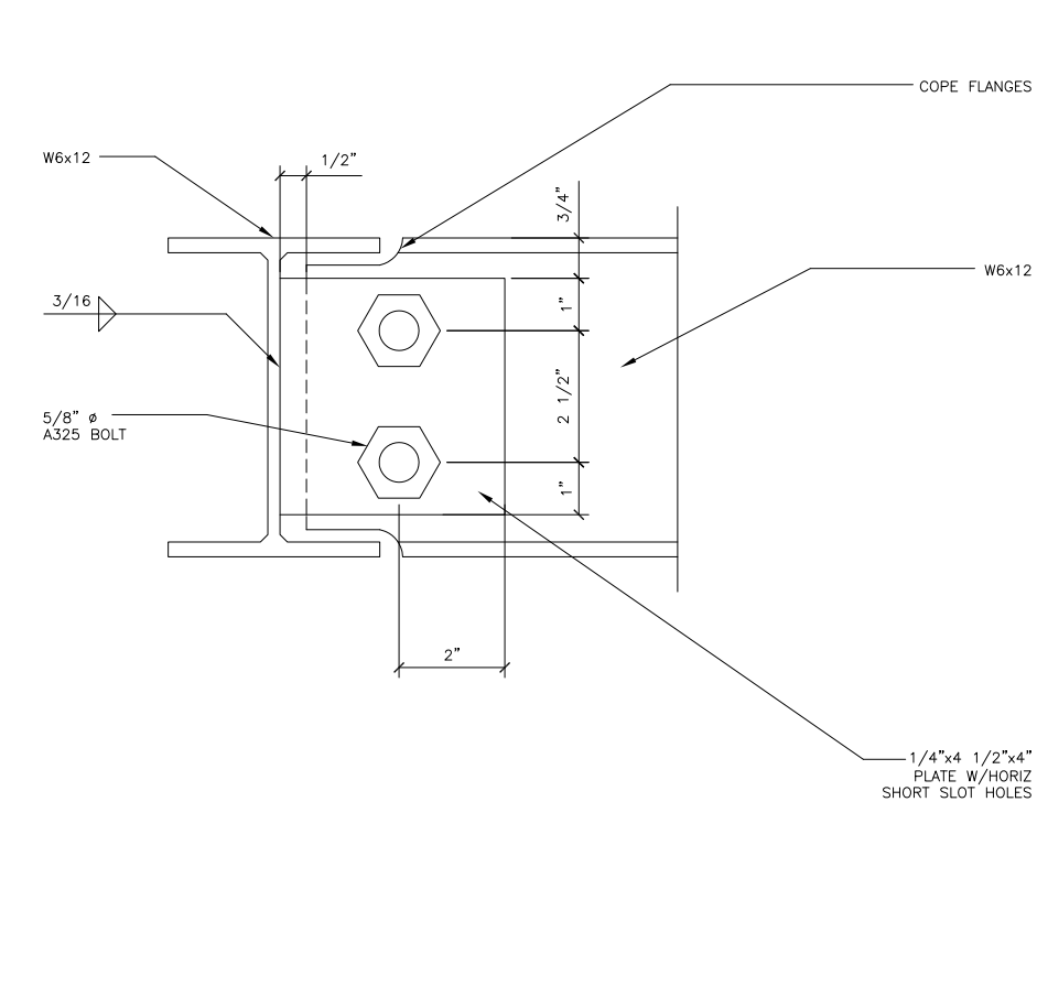
2 W6 TO W6 DETAIL 0859/X_A803-2 SCALE: 0 3" 6"
