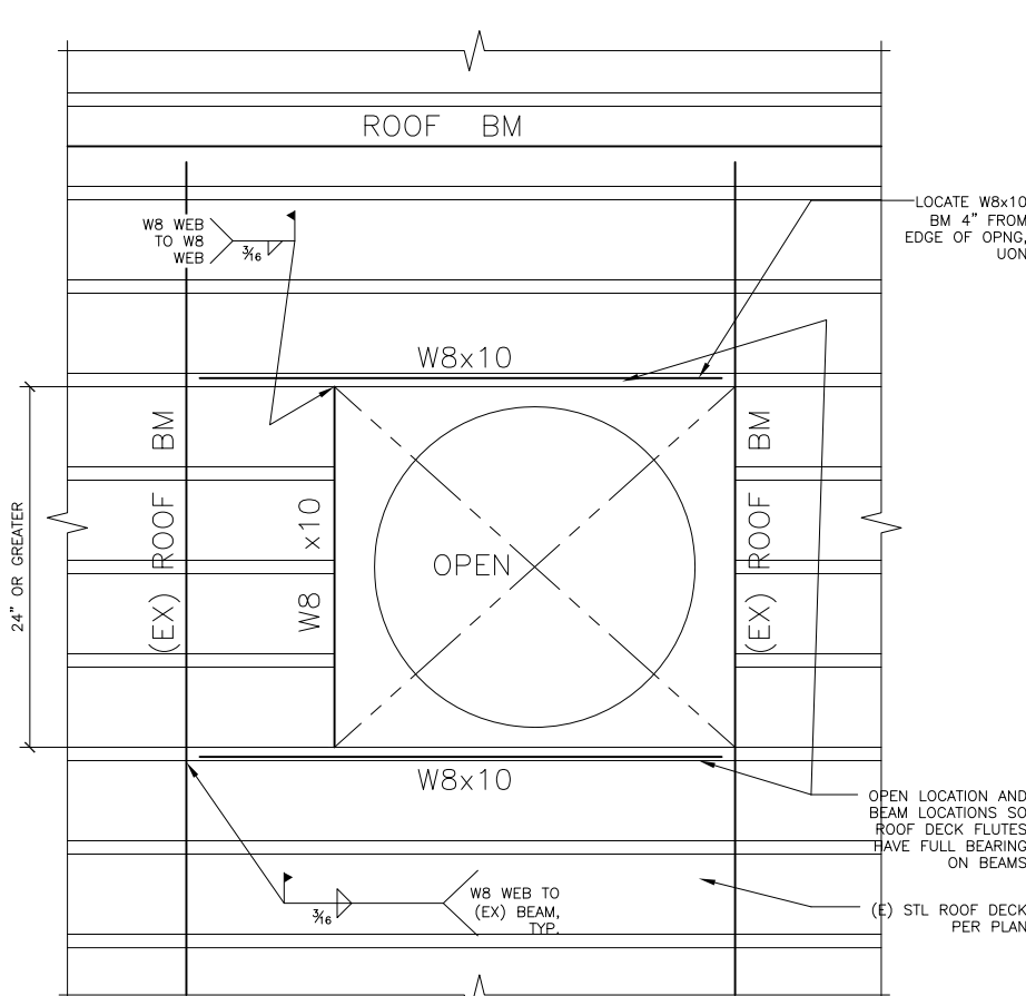
2 TYPICAL ROOF OPENING 0859/A804-2 SCALE: 0 6" 1' 2'
