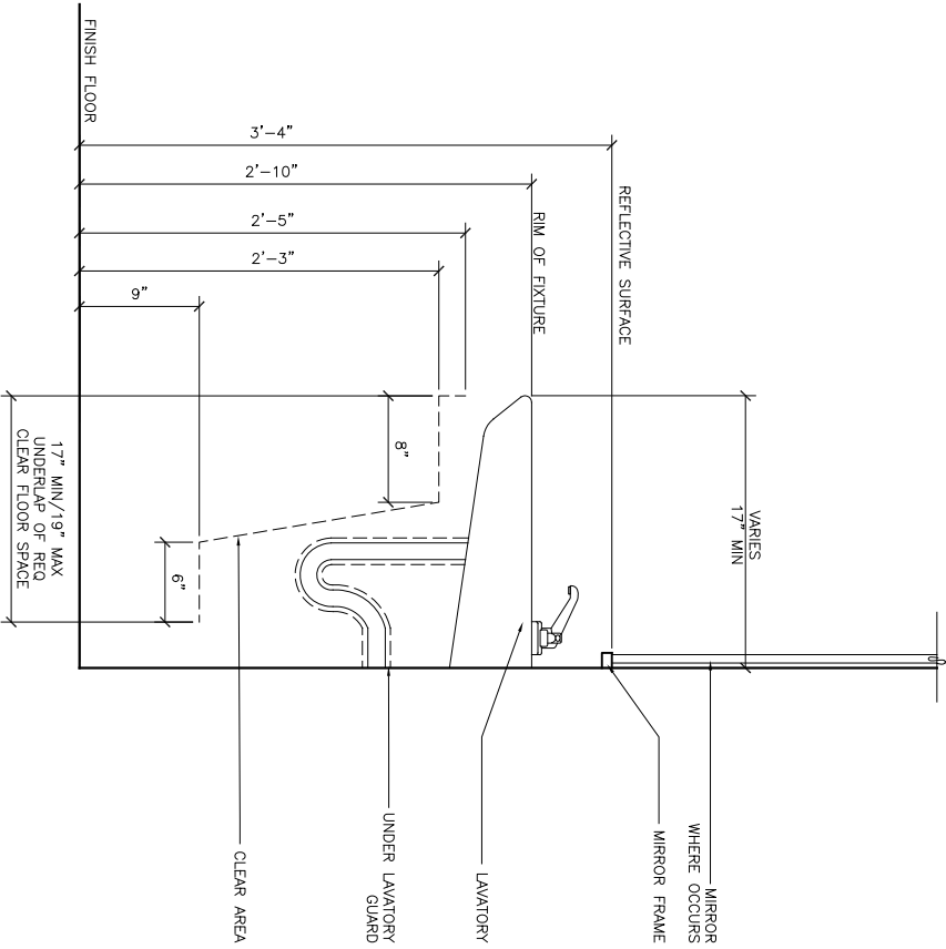
2 ACCESSIBLE LAVATORY
