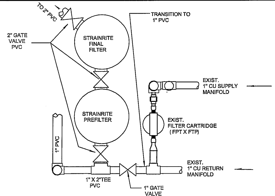
PLAN BAG FILTER LAYOUT D
