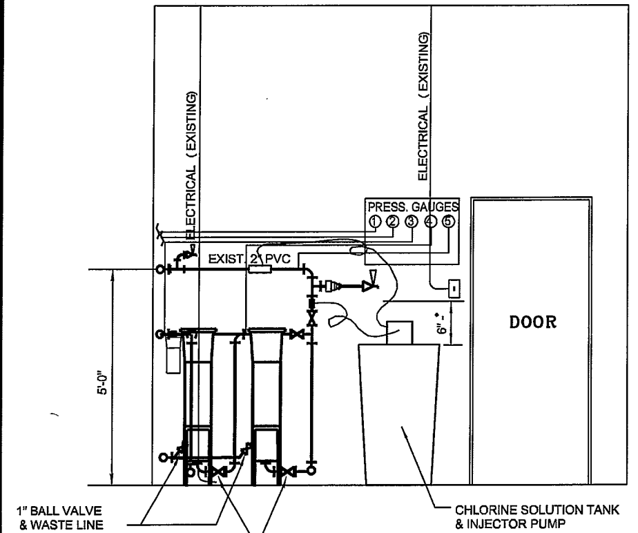
FRONT WALL ELEVATION C
