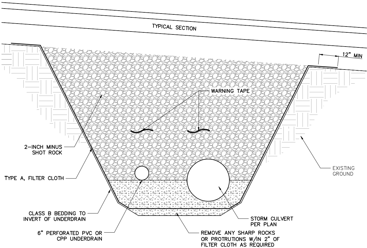
3 UNDERDRAIN DETAIL NTS
