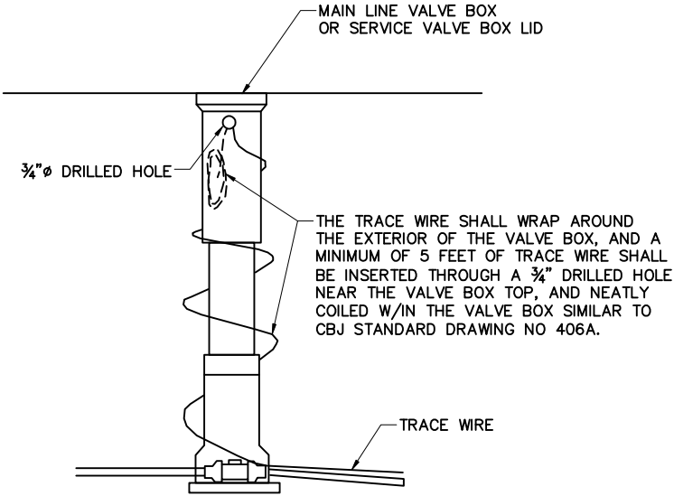
1 MAIN LINE VALVE & SERVICE VALVE TRACE WIRE TERMINATION DETAIL NTS
