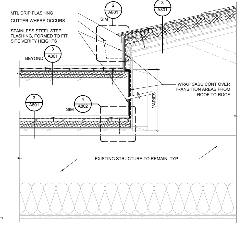
5 ROOF TRANSITION 21037 - X_A802-5 SCALE: 0 6\"/>
