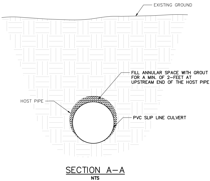
1 STORM DRAIN - SLIPLINE NTS
