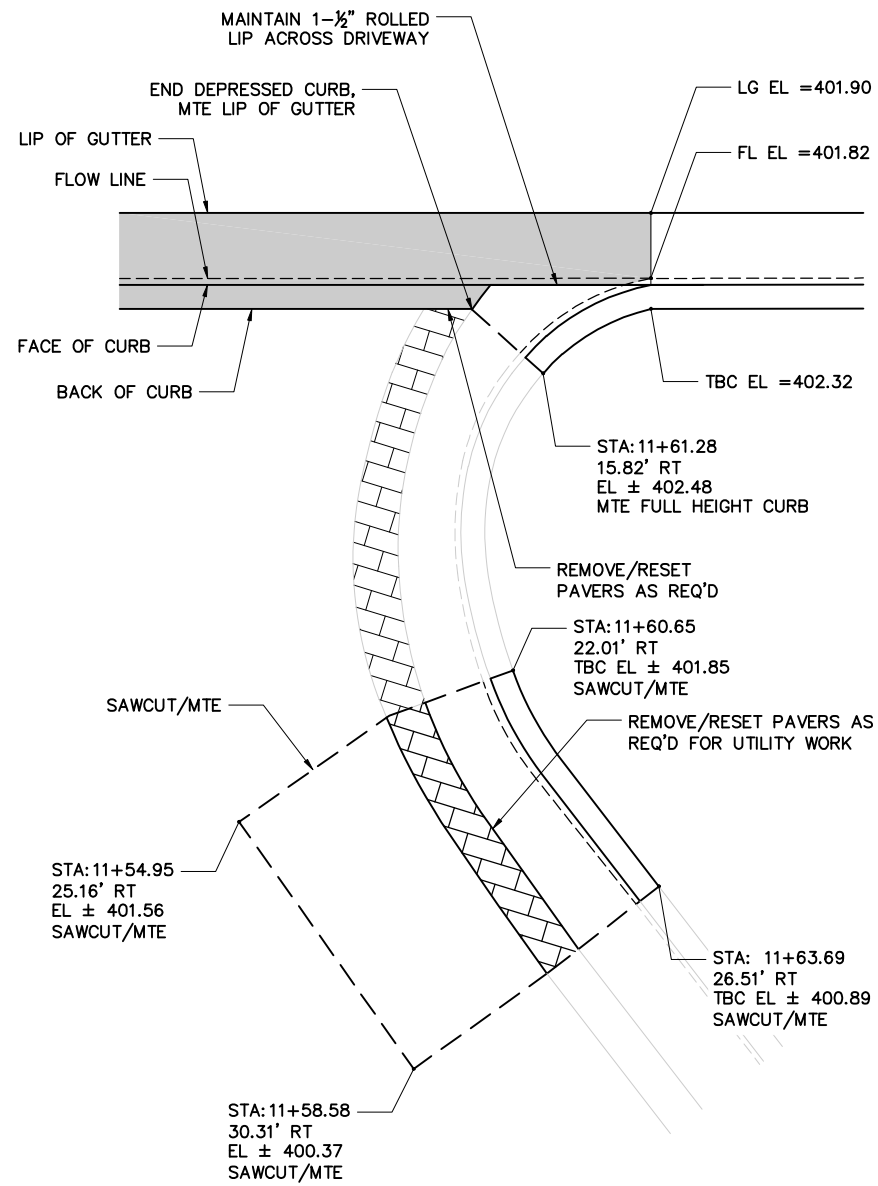
1 #3000 MATCH TO EXISTING CURB NTS
