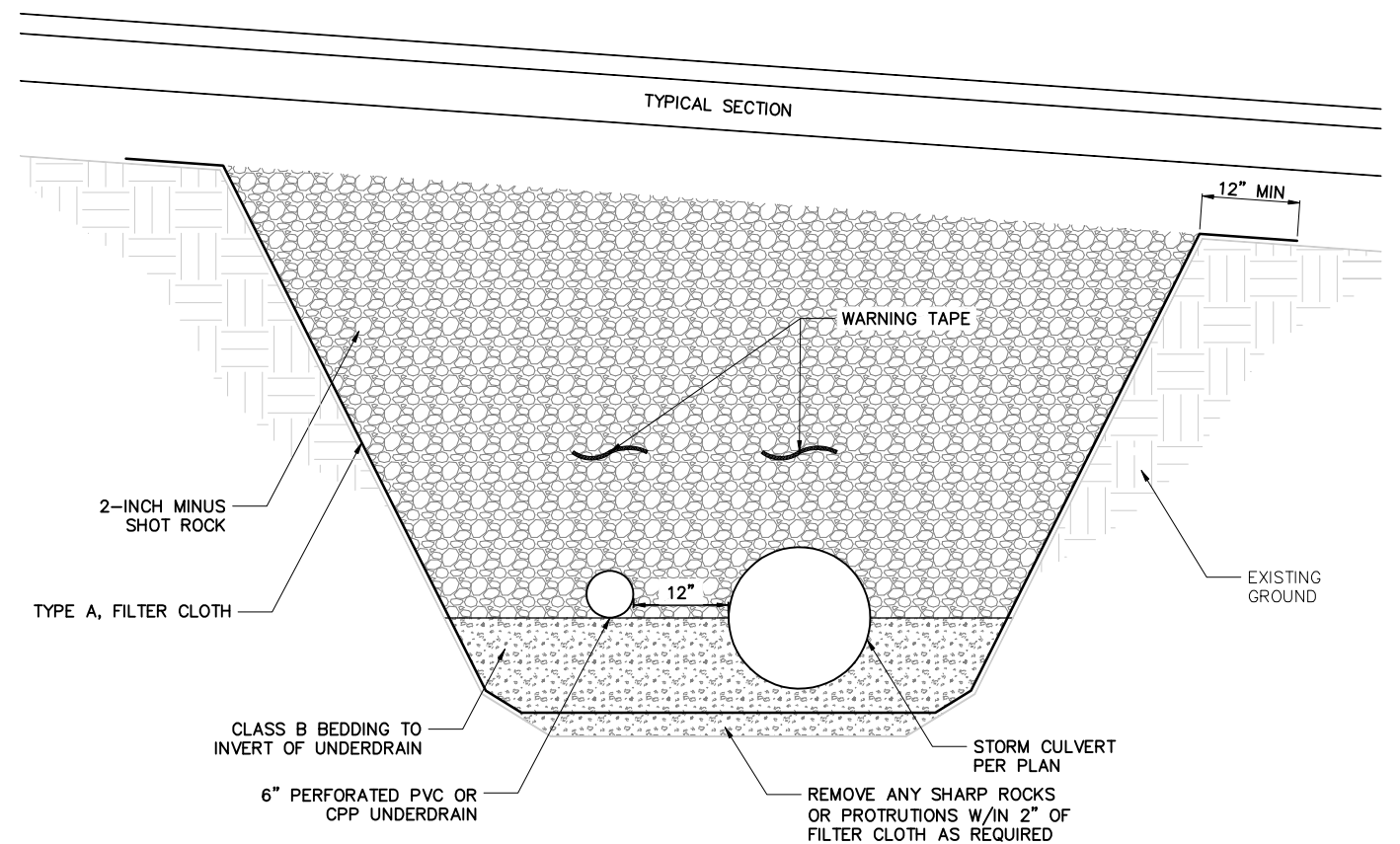
3 STORM DRAIN TRENCH WITH UNDERDRAIN NTS
