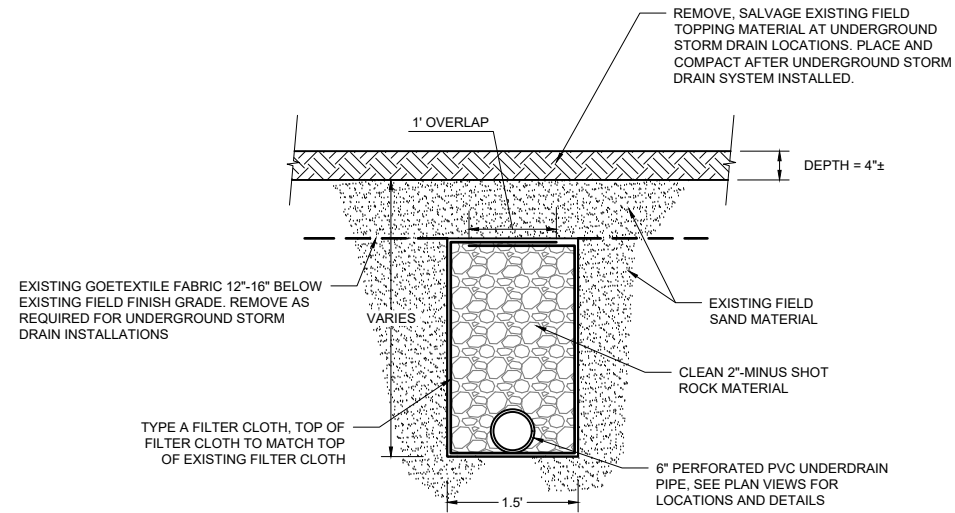
② TYPICAL FIELD UNDERDRAIN DETAIL N.T.S.
