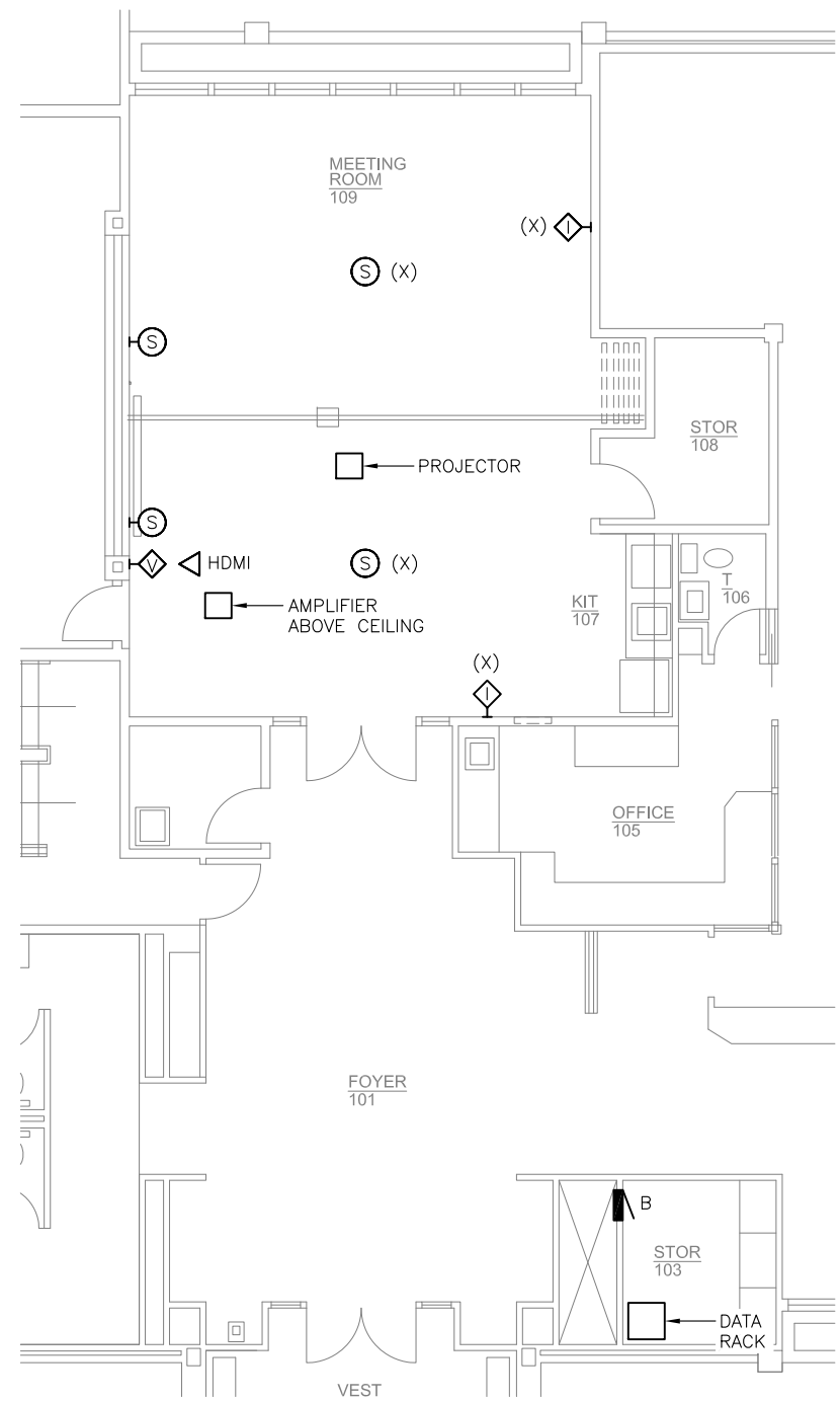
1 ELECTRICAL DEMOLITION PLAN SCALE: 0 2' 4' 8'
