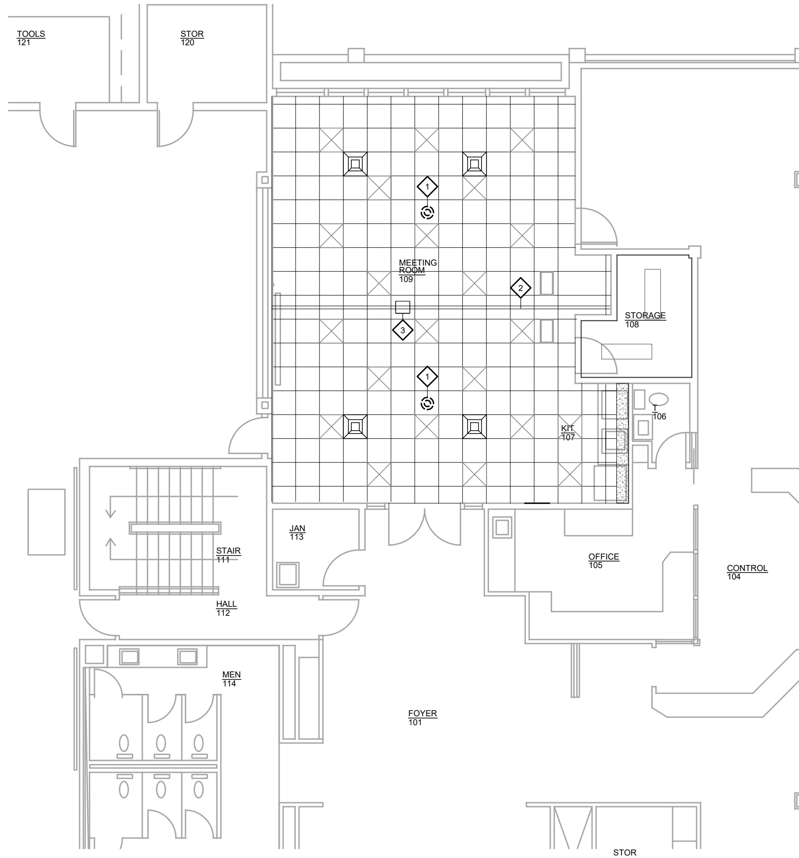
1 MAIN FLOOR ENLARGED REFLECTED CEILING PLAN
