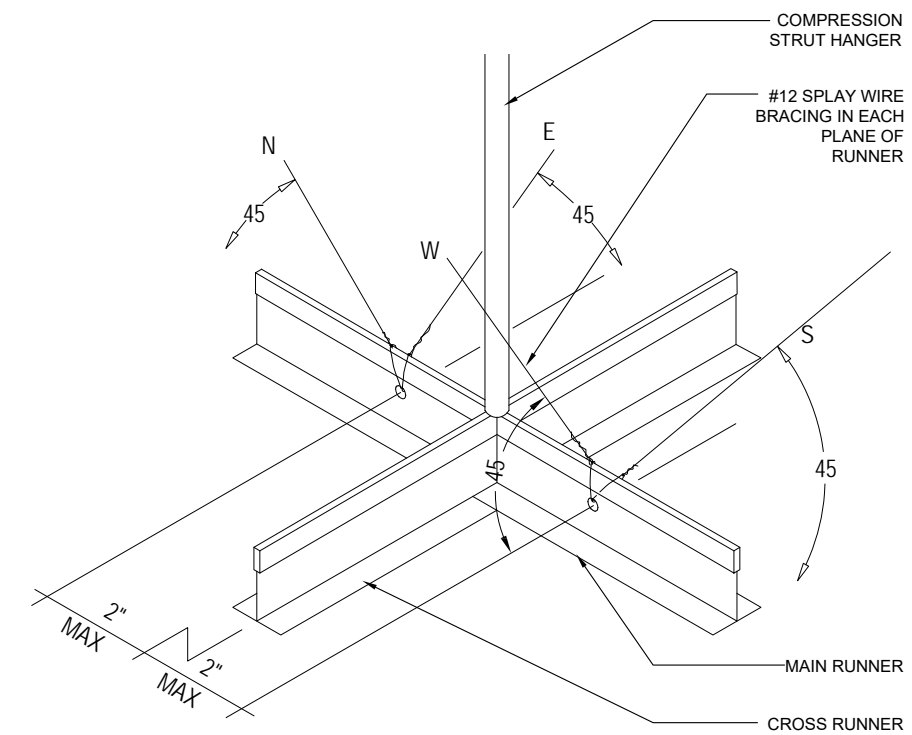
NOTE: ACOUSTICAL PANEL CEILINGS, LIGHT FIXTURES AND DIFFUSERS ARE TO BE IN COFORMANCE WITH IBC 1621.2.5 (SEISMIC DESIGN CATEGORY D) AND CISCA STANDARDS 2 ADD ALTERNATE: TYP CEILING BRACING 20014/A901-2 SCALE: 0 3" 6" 1'
