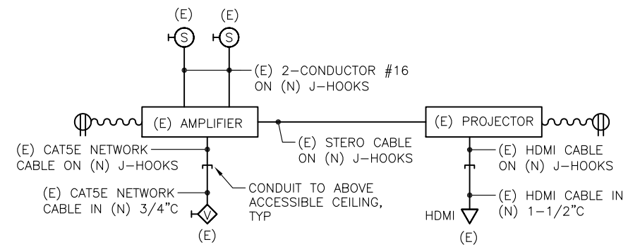
3 AUDIO SYSTEM SINGLE LINE DIAGRAM
