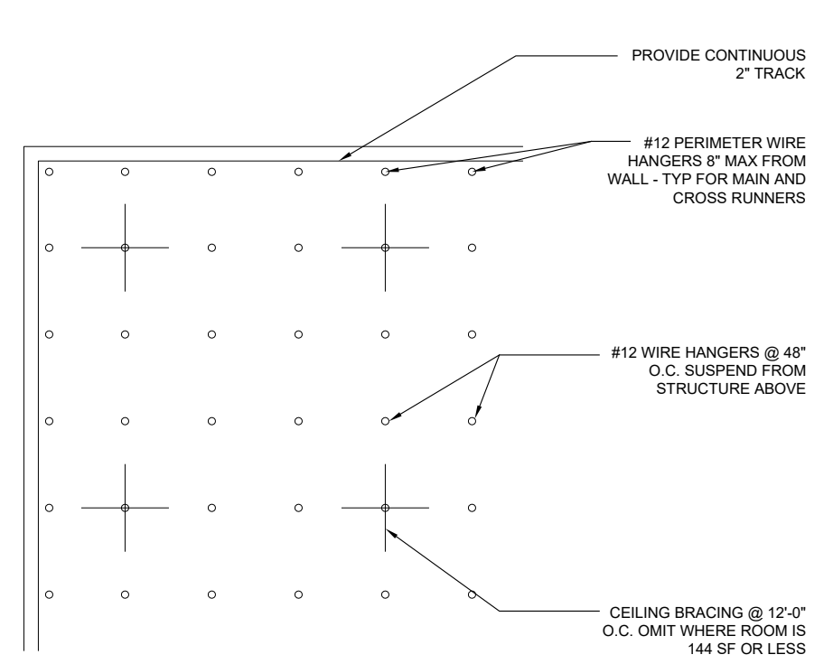
3 ADD ALTERNATE: TYP BRACING LAYOUT 20014/A901-3 SCALE: 0 3" 6" 1'
