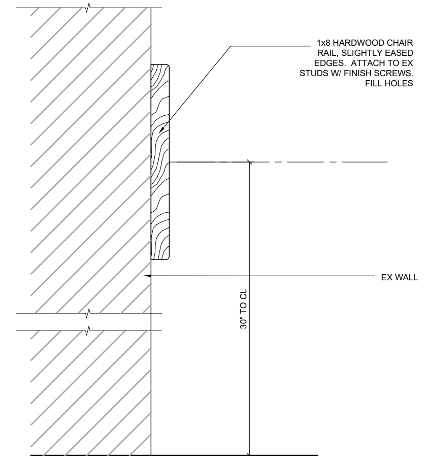
3 CHAIR RAIL 20014/A901-5 SCALE: 0 3" 6"
