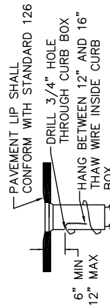
THAW WIRE INSTALLATION DETAIL
