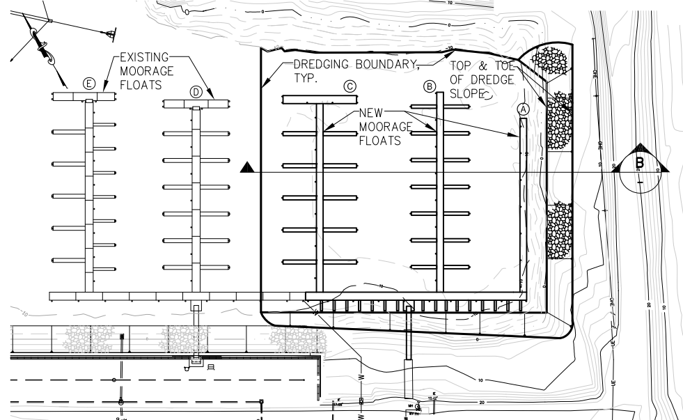
HARBOR DREDGING - PLAN
