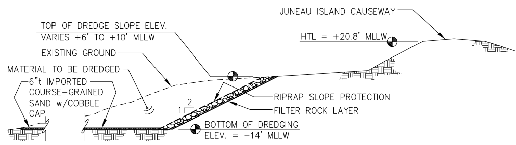
A HARBOR DREDGE w/CAP - SECTION
