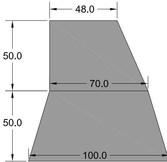
PLAN VIEW
