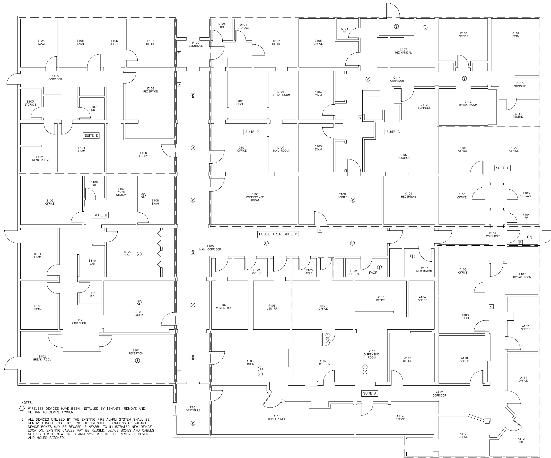
1 FLOOR PLAN - FIRE ALARM DEMOLITION SCALE: 0 2' 4' 8' 16'
