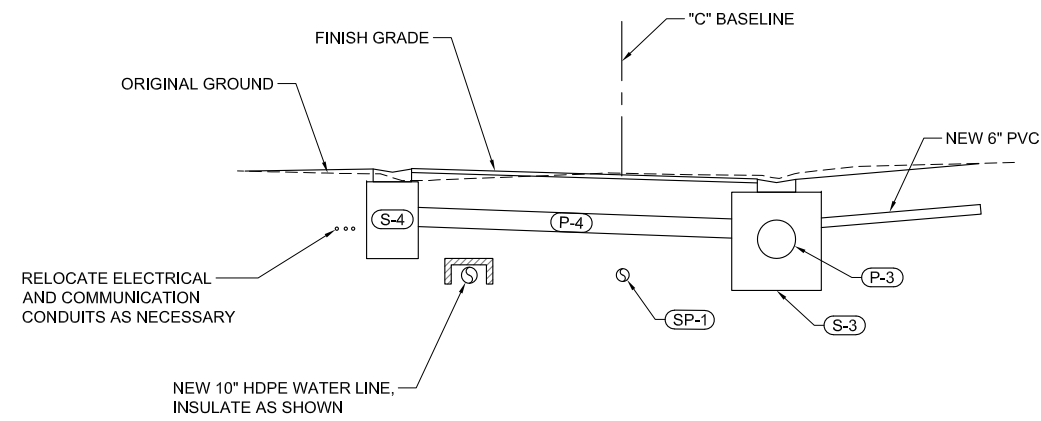
2 PIPE P-4 PROFILE, VIEW LOOKING UP STATION C104 SCALE: NTS
