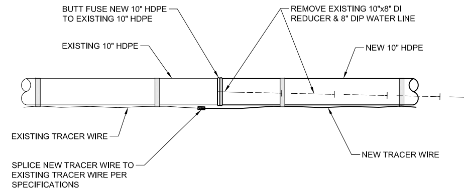
1 STA "C" 10+54, 12' RT. WATER LINE CONNECTION DETAIL C103 SCALE: NTS
