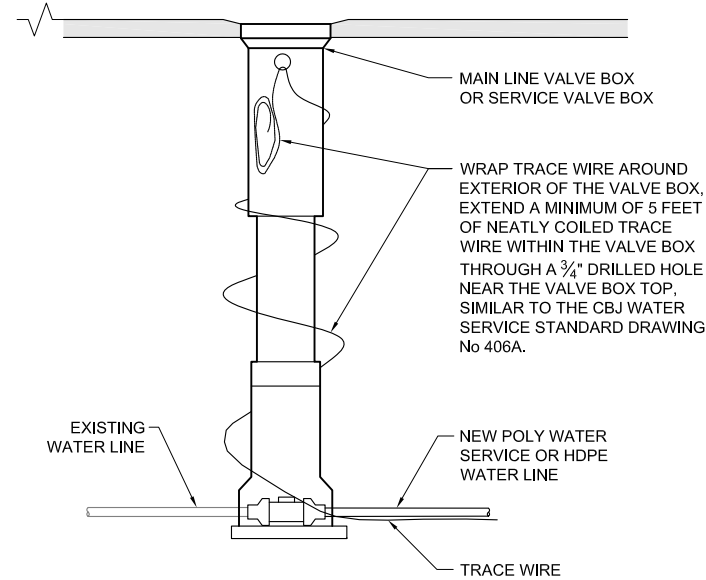
3 MAIN LINE VALVE & SERVICE VALVE TRACE WIRE TERMINATION DETAIL C102 SCALE: NTS
