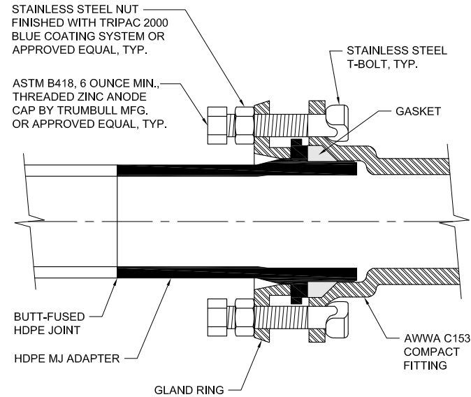
2 TYPICAL HDPE MJ CONNECTION TO DI FITTING C102 SCALE: NTS
