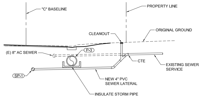
3 8213 CEDAR DRIVE SEWER LATERAL PROFILE VIEW LOOKING UP STATION C104 SCALE: NTS
