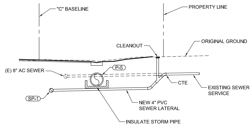
4 8209 CEDAR DRIVE SEWER LATERAL PROFILE VIEW LOOKING UP STATION C104 SCALE: NTS
