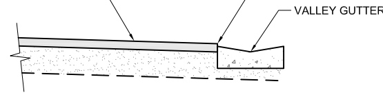
1 GRADE CLARIFICATION DETAIL C400 SCALE: NTS
