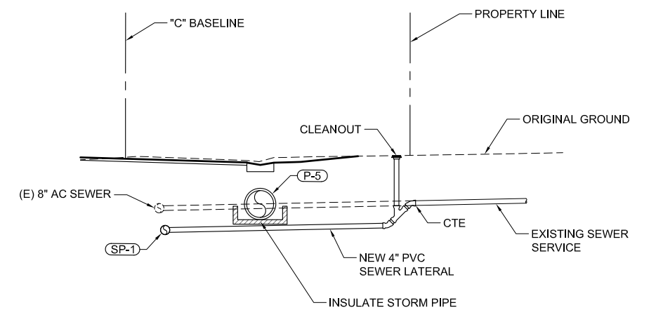
5 8205 CEDAR DRIVE SEWER LATERAL PROFILE VIEW LOOKING UP STATION C104 SCALE: NTS
