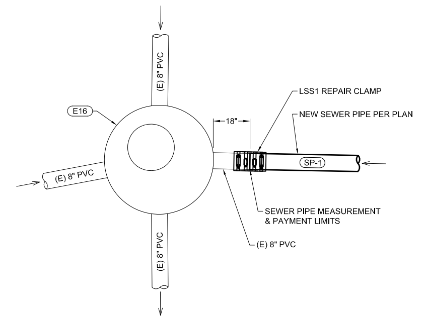
7 STA "C" 10+06.4, 1.6' LT. SEWER LINE CONNECTION DETAIL C102 SCALE: NTS
