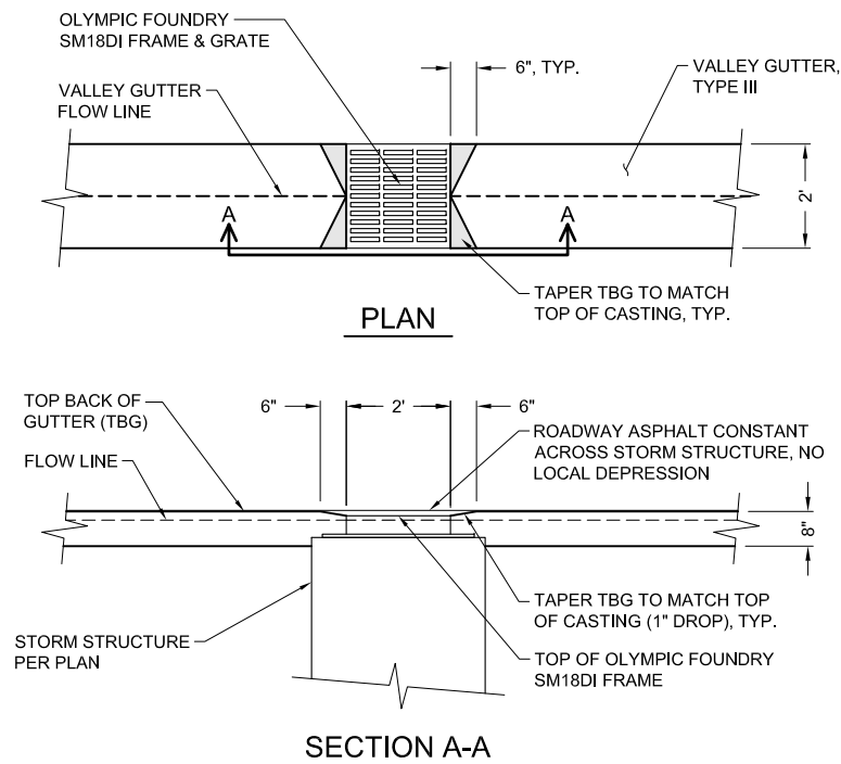
5 VALLEY GUTTER TRANSITION AT CURB INLET DETAIL C102 SCALE: NTS
