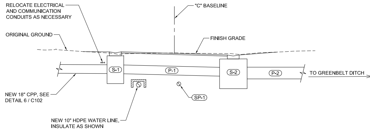
1 PIPE P-1 PROFILE, VIEW LOOKING UP STATION C104 SCALE: NTS
