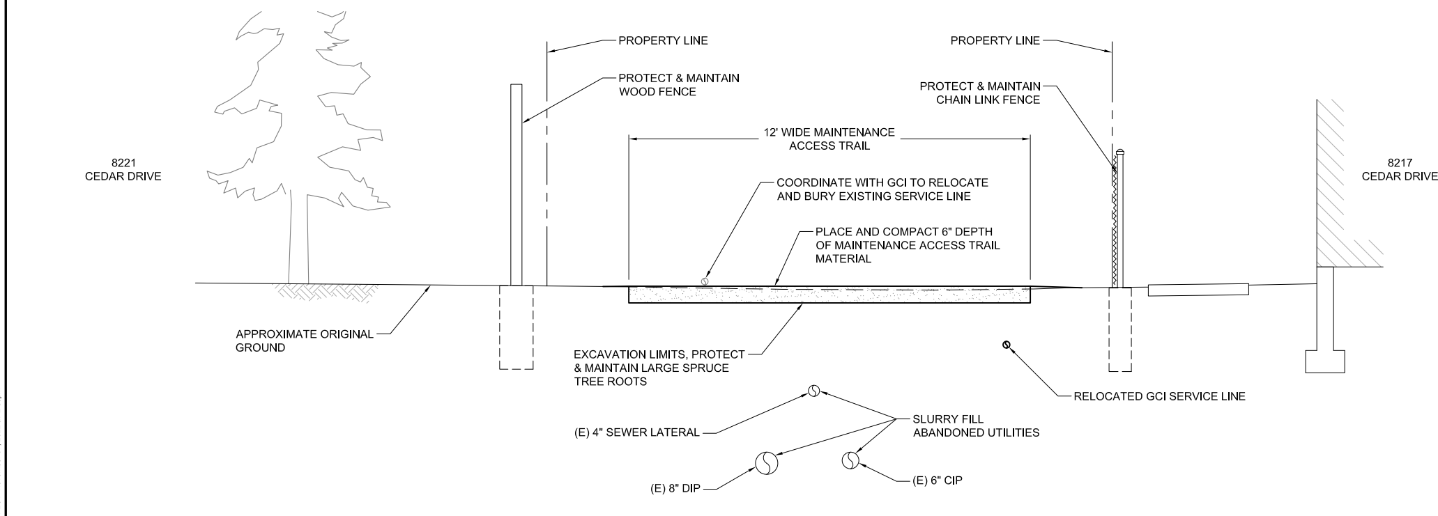
2 MAINTENANCE ACCESS TRAIL TYPICAL SECTION C101 SCALE: NTS
