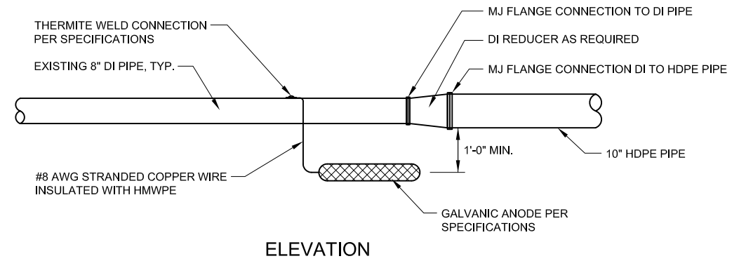
1 GALVANIC ANODE INSTALLATION FOR EXISTING METALLIC PIPE CONNECTIONS OR LEAK REPAIR LOCATIONS DETAIL C102 SCALE: NTS
