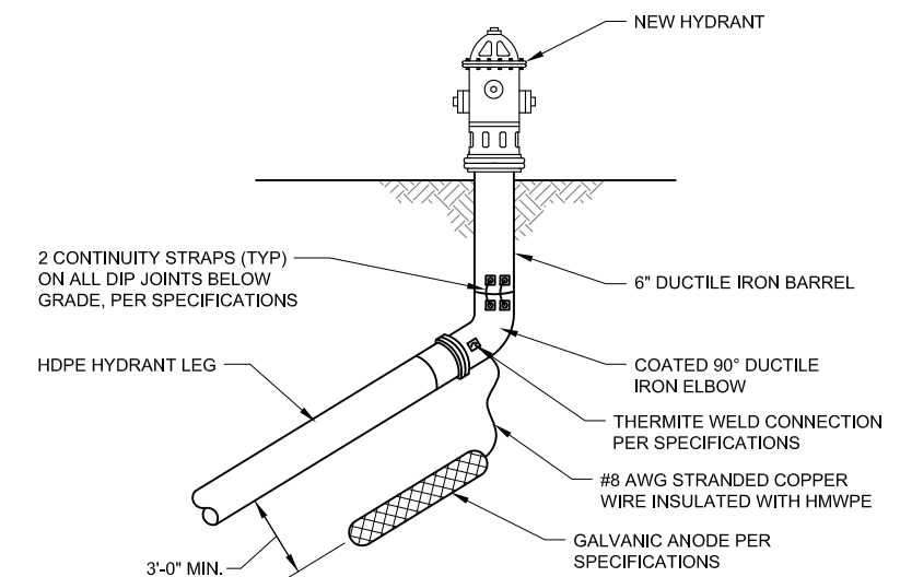
2 GALVANIC ANODE INSTALLATION AT HYDRANT ASSEMBLIES WITH HDPE C102 SCALE: NTS
