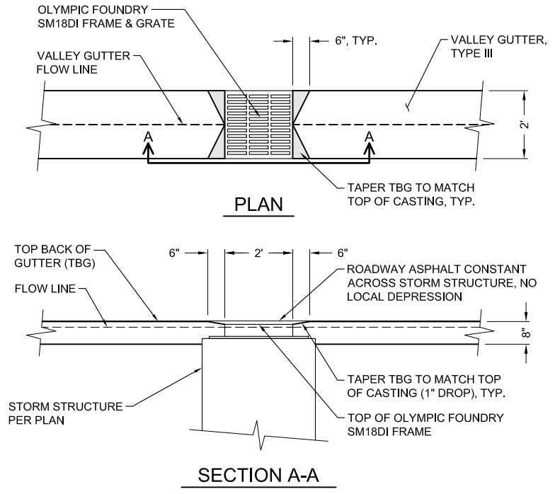
6 VALLEY GUTTER TRANSITION AT CURB INLET DETAIL C101 SCALE: NTS
