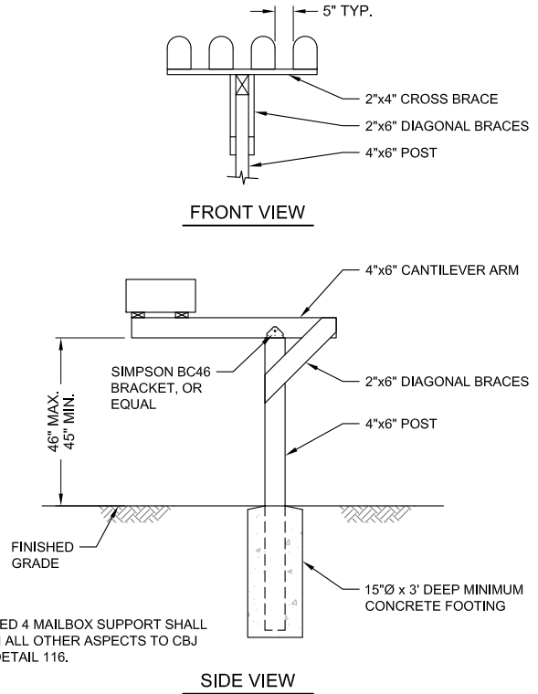
8 CANTILEVERED 4 MAILBOX SUPPORT DETAIL C101 SCALE: NTS
