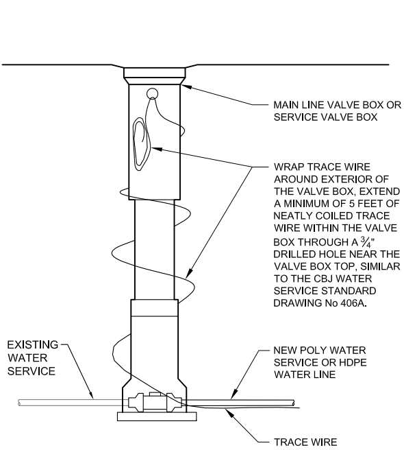
5 MAIN LINE VALVE & SERVICE VALVE TRACE WIRE TERMINATION DETAIL C101 SCALE: NTS
