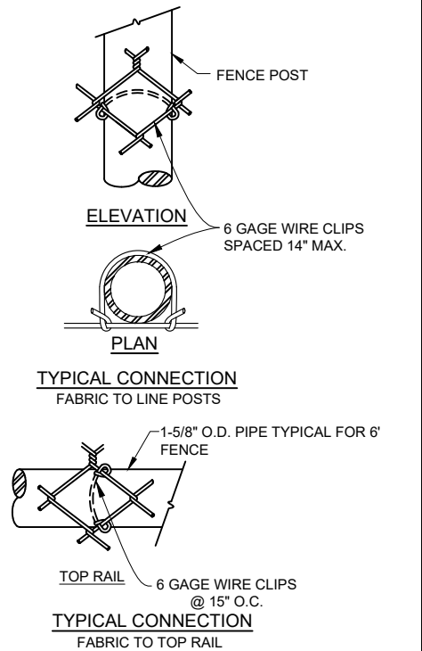
G FENCE DETAILS C401 NTS
