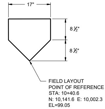
C HOME PLATE DETAIL C400 NTS
