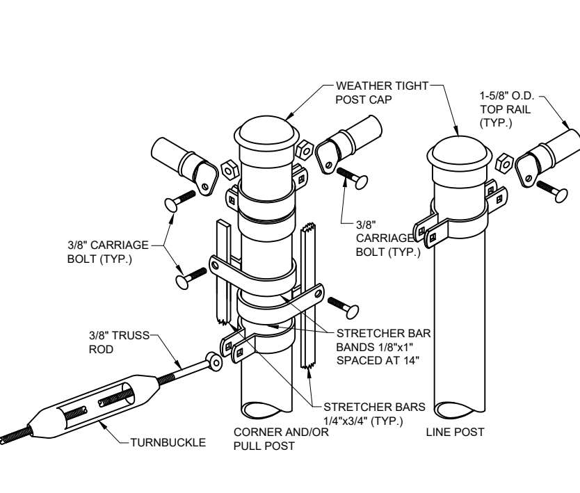
F PIPE POST TOP DETAIL C401 NTS
