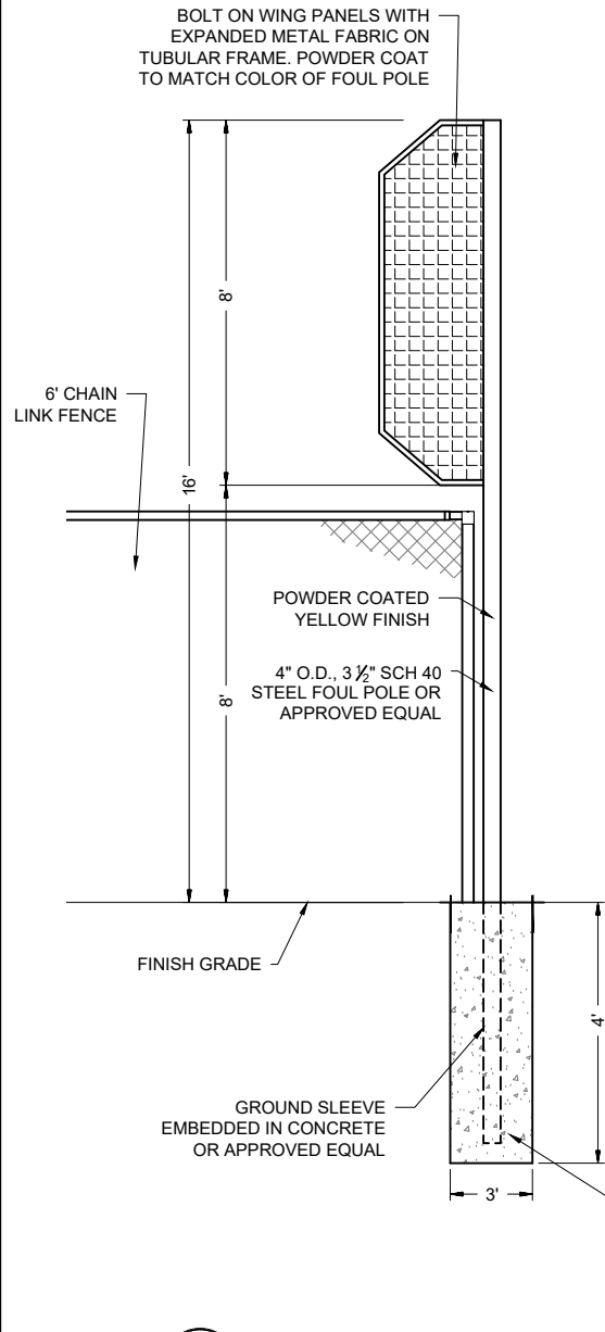
A 16' FOUL POLE WITH WING C400 NTS
