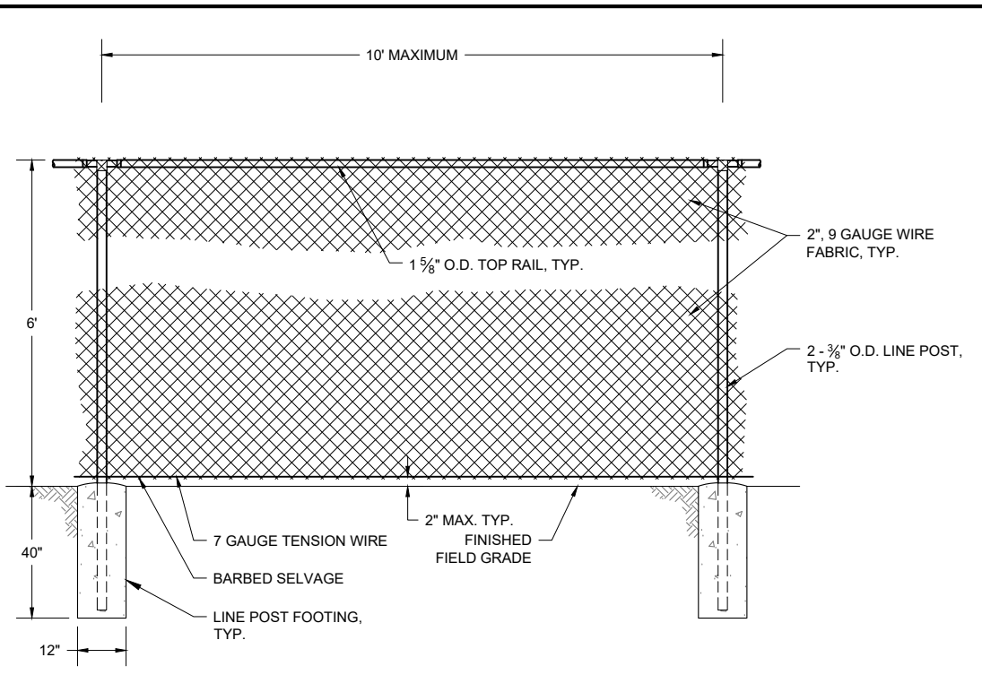
C TYPICAL FENCE ELEVATION C401 NTS
