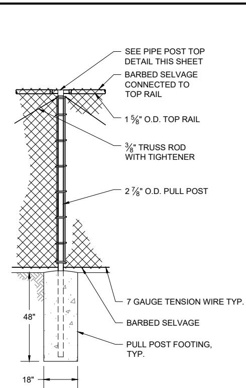
B TYPICAL PULL POST DETAIL C401 NTS NOTE: PULL POSTS SHALL BE LOCATED AT 150' MAXIMUM INTERVALS.
