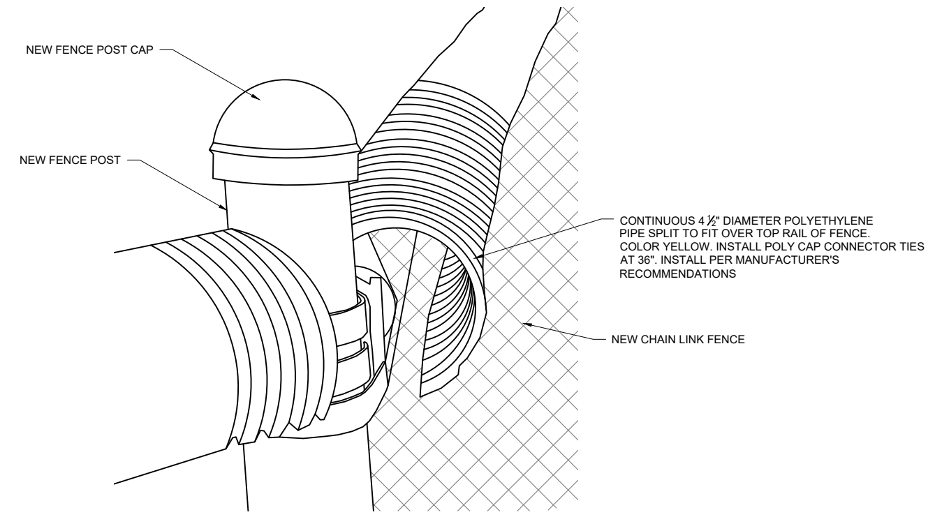
B POLY CAP FENCE TOP PROTECTOR DETAIL C400 NTS
