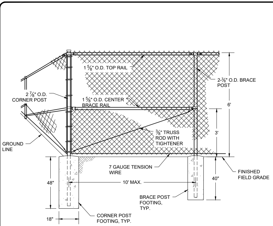
A TYPICAL CORNER TERMINAL DETAIL C401 NTS
