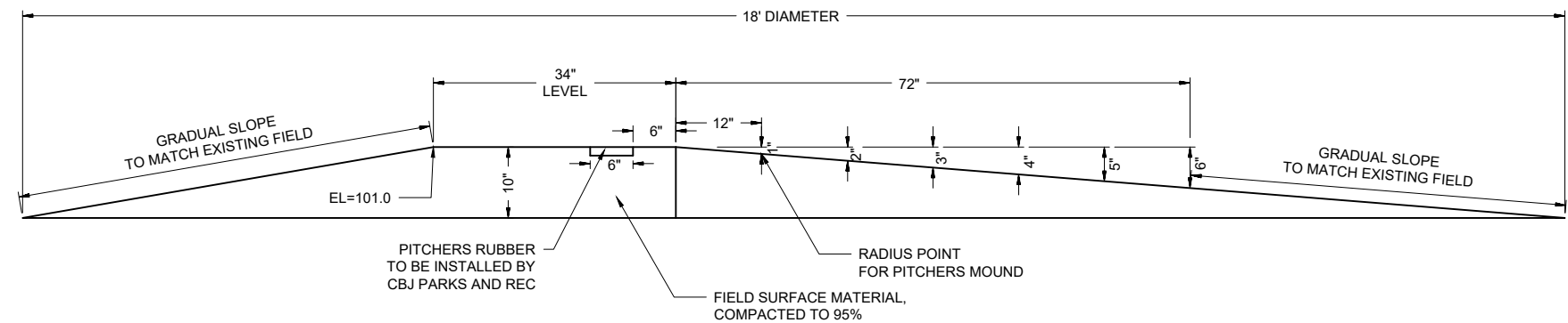
E PITCHING MOUND SLOPE DETAIL - SECTION A-A C400 NTS
