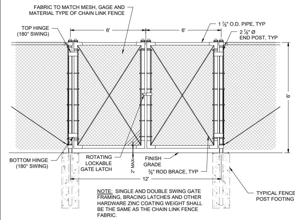
D 6' DOUBLE SWING GATE C401 NTS
