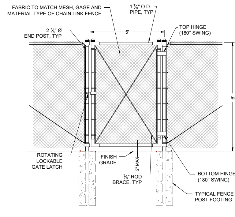
E 5' SINGLE SWING GATE C401 NTS
